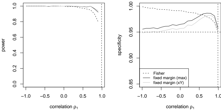
Figure 4. Performance curves: dashed lines for Fisher methods (black) and solid lines for fixed margin (black: maximum, grey: fixing X). Moderate variance \sigma_\rho = 0.2 ; Medium sizes; 2% contamination; departures w.r.t. \rho_0 = 0.99 , n_{sim} = 400 .
