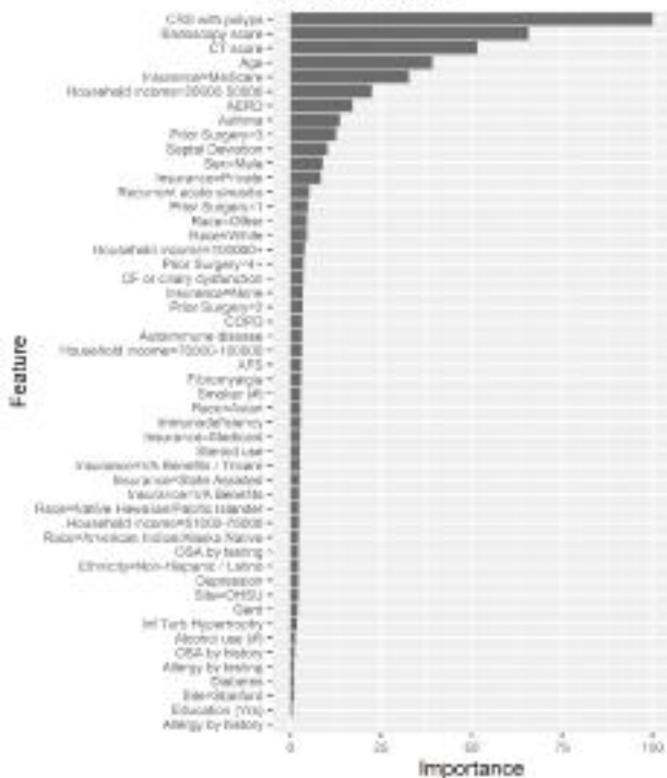
Random Forest
