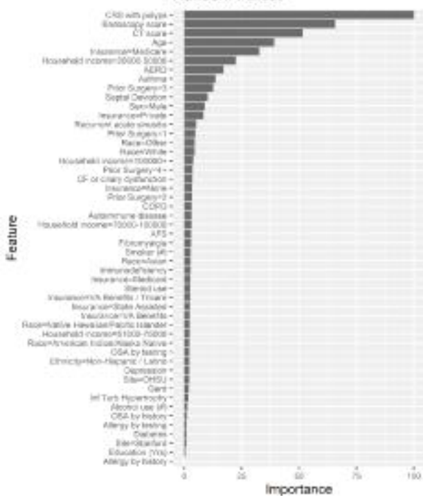
Random Forest
