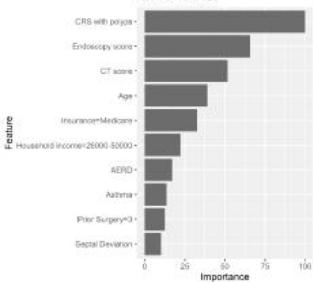
Random Forest
