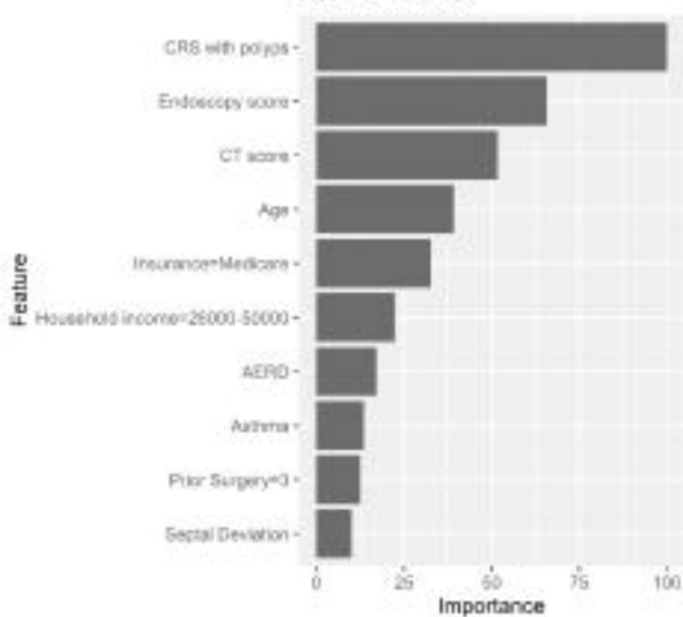
Random Forest
