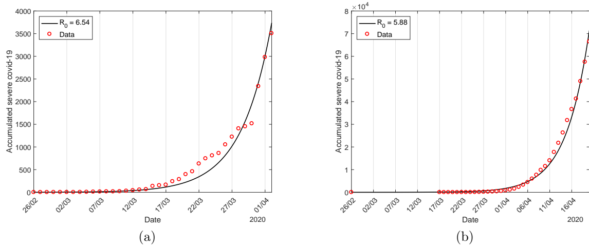
Figure 4: The estimated curve \Omega and the observed accumulated cases for São Paulo State (a) and Spain (b).
