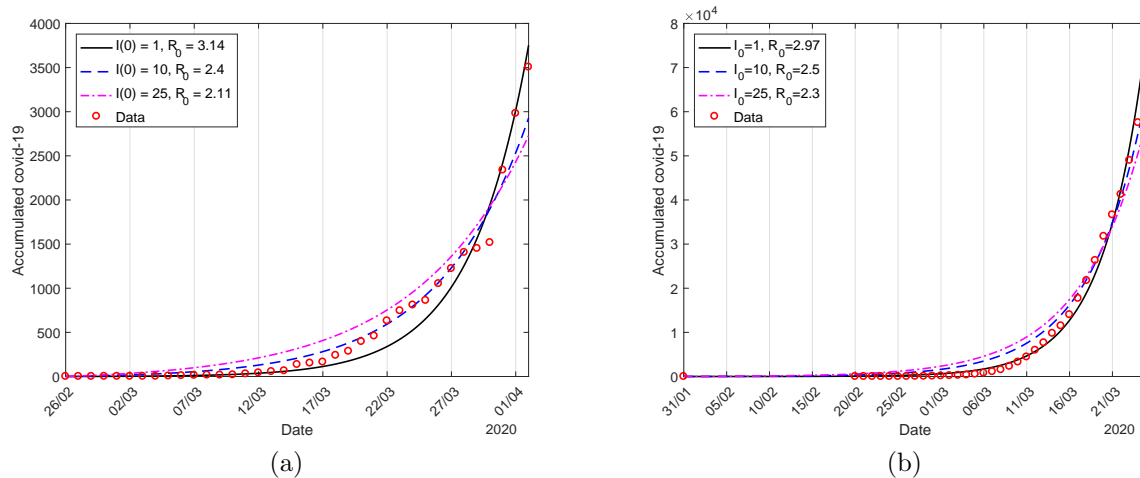
Figure 1: The estimated curve \Omega for São Paulo (a) and Spain (b) with three different initial conditions I(0) = 1 (continuous curve), 10 (dashed curve), and 25 (dashed and dotted curve).
