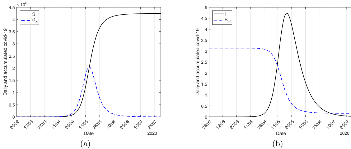
Figure 2: The estimated curve of \Omega and the daily curve \Omega_d (a), and the epidemic curve I and effective reproduction number R_{ef} (b).
