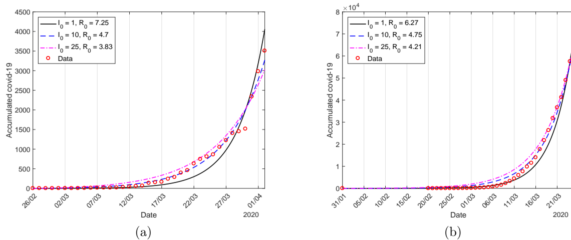
Figure 3: The estimated curve \Omega for São Paulo (a) and Spain (b) with three different initial conditions I(0) = 1 (continuous curve), 10 (dashed curve), and 25 (dashed and dotted curve).
