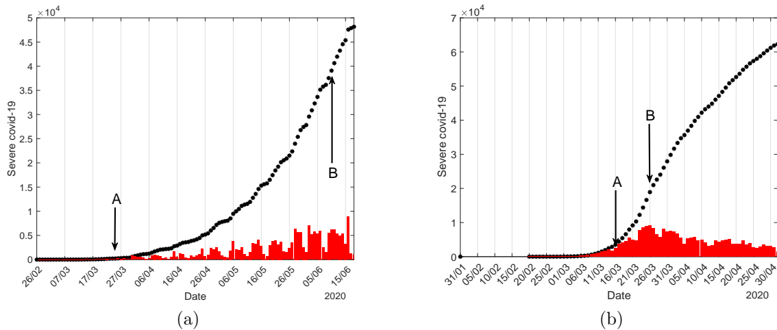
Figure 5: The daily (bars) and the accumulated (points) severe covid-19 cases in São Paulo State (a) and Spain (b), where A indicates the time at which quarantine was introduced, and B indicates the inflection time.
