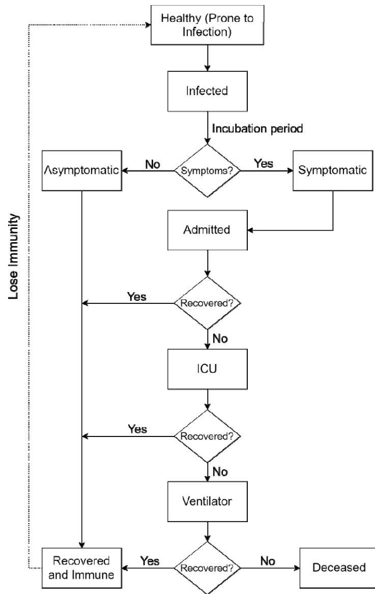
Figure 1: State Chart
