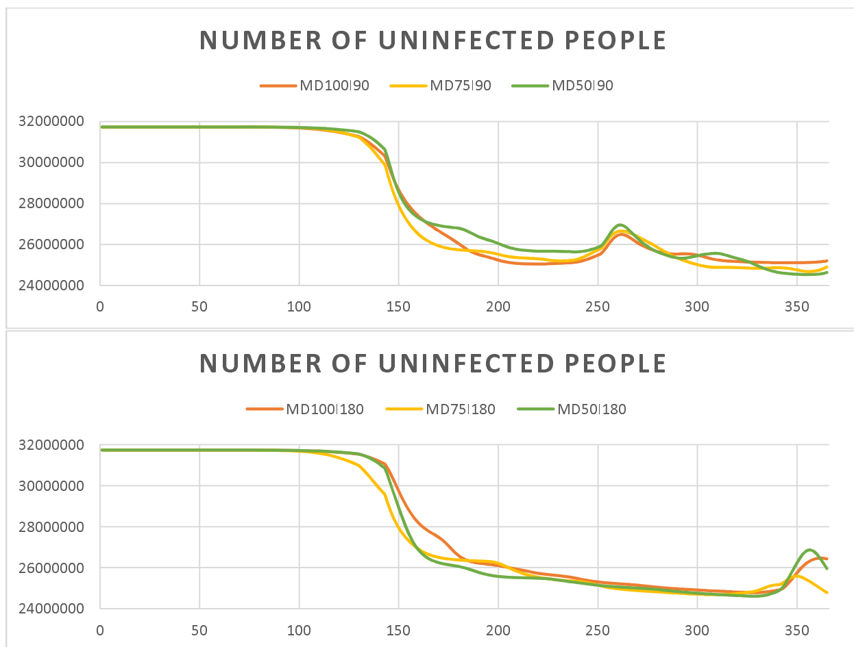
Figure 2 a): Number of Uninfected people (90 days immunity scenarios); b) Number of Uninfected people (180 days immunity scenarios)
