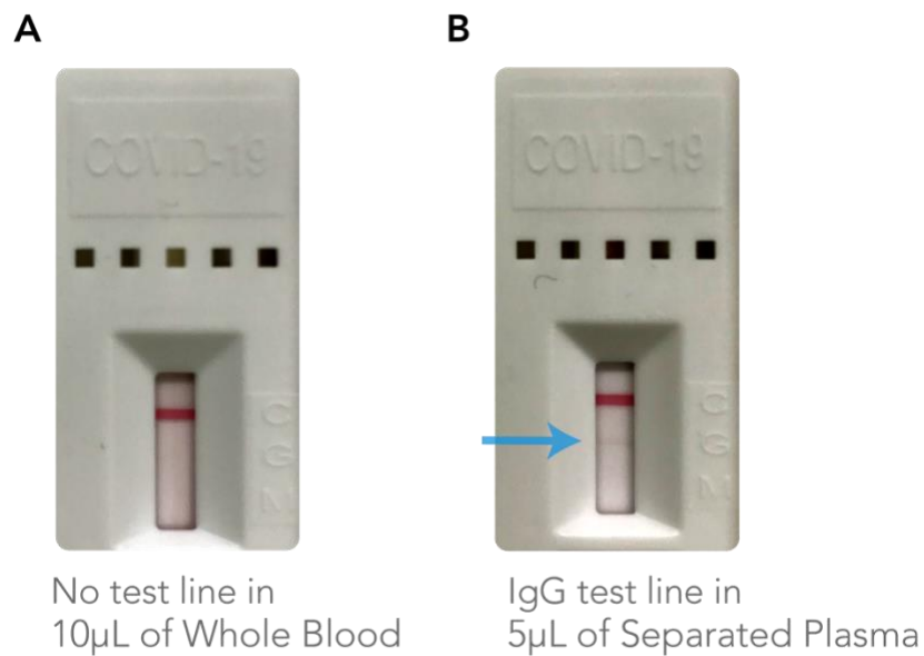
Figure 1: Example of an incorrectly assessed False Negative test in whole blood. A) Test result from using whole blood and B) test result using H.E.R.M.E.S plasma from the same sample. A faint IgG response is noted by the arrow.
