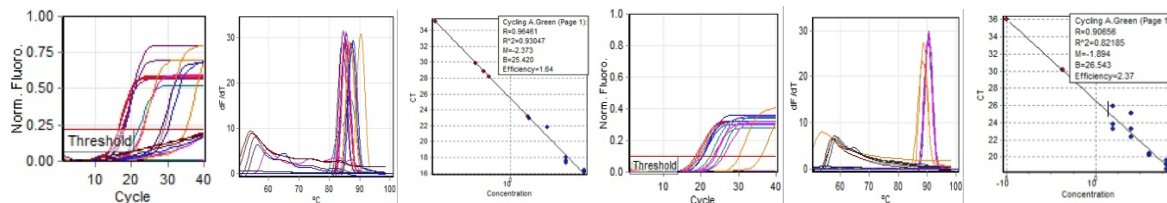
157 158 Figure 4a-f (left to right): E-gene amplification, melt, and standard curve; N-gene 159 amplification, melt, and standard curve.
