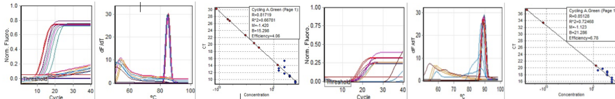
148 149 Figures 3a-f (left to right): E-gene amplification, melt, and standard curve; N-gene 150 amplification, melt, and standard curve.
