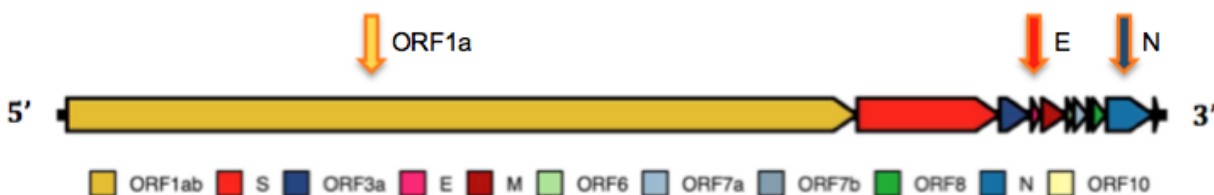
Figure 1. SARS-CoV-2 genome and subunit arrangement with primer locations
