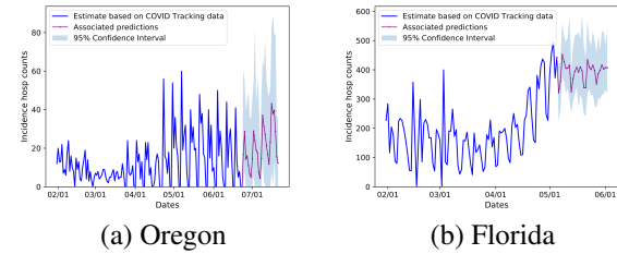
Figure 3: Two examples of finer grained reporting patterns captured by DEEPCOVID. Note the dips in reporting for weekends.
