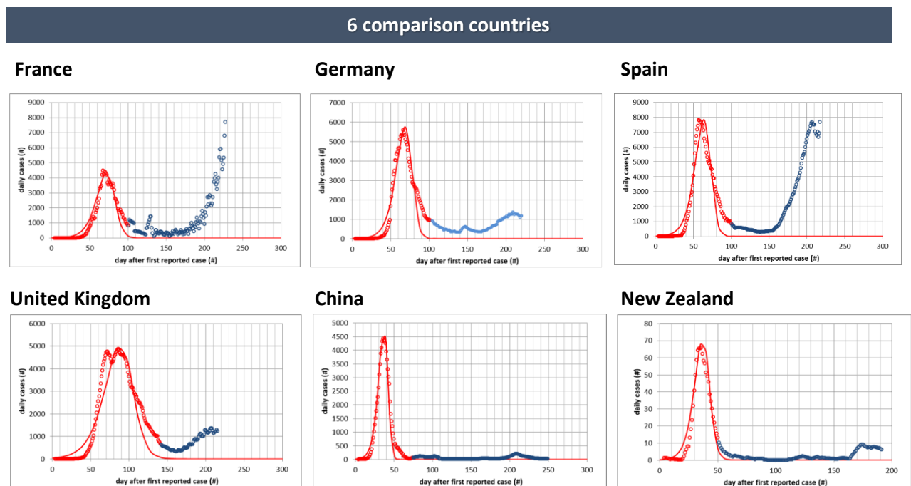
Figure 3: Daily reported new cases of COVID-19 (based on a 7-day rolling average, the dots) for 6 comparison countries, with best-fit curves for first peak in these countries (the red line). Note that the red dots are datapoints that are included in the fits and the blue dots represent datapoints which are not used in fitting.
