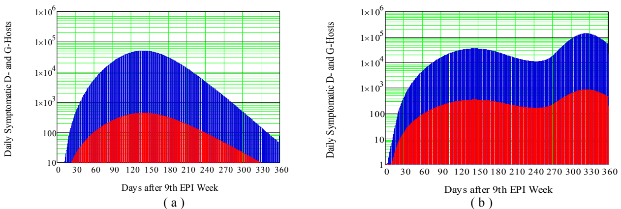
Figure 7. Estimated evolutions of symptomatic infected host to SARS-CoV-2 original D-form and G-variant are presented in (a) and (b). Red and blue shades present respectively the evolution of D and G exposed hosts to SARS-CoV-2. (a) Preserving NPIs. (b) Progressive release of NPIs as reported world wise during the last quarter of 2020, and as modeled in Fig.1.
