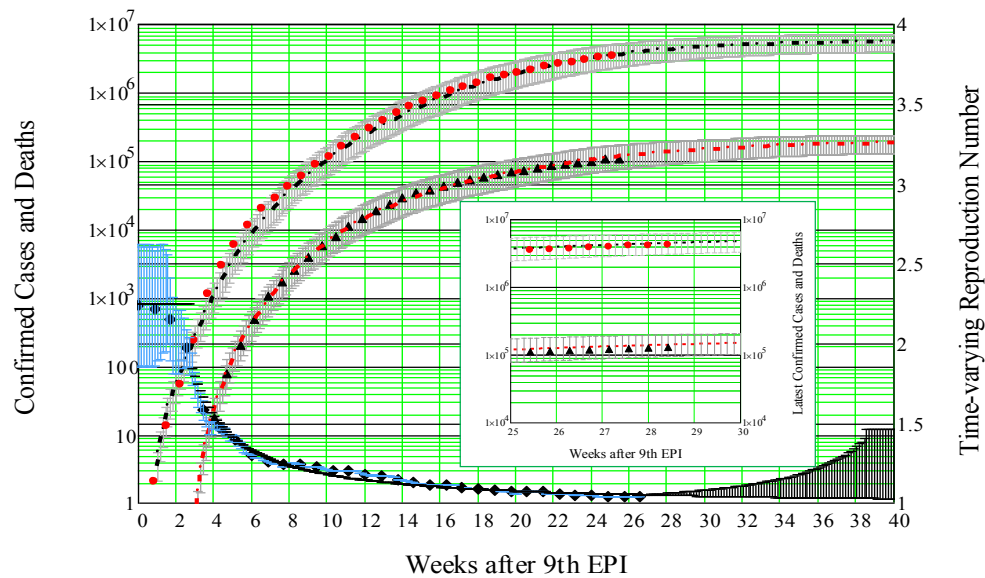
Figure 1. Data on confirmed cases and fatalities are shown by solid red circles, and solid black triangles respectively. Error bars account for the RMS values on the SEIR parameters. The fitting values to SEIR model are: N = 6.10^7 , \beta_0 = 1.265 , \sigma_D = 0.25 , \sigma_G = 2\sigma_D , R_0 = 2.25 and \alpha_s = 0.47 \pm 0.09 . Average values and error bars (vertical in black) for infected individuals, and fatalities are shown respectively in solid red circles and solid black triangles. The mean fitting to the infected individuals (logarithmic scale) presents standard deviation SD = 0.08 . Right vertical axis shows: (a) the mean time-varying R(t) (data from Table 1 - solid blue diamond) 11 , vertical bars represent 5 to 95% CRI; (b) R(t > 9 + 27 \text{ EPI}) estimated forecasts (shaded black area) preserving or releasing the NPIs. Data points for the last three weeks (Figure Inset - solid circles and triangles) were added after the model was complete, granting confidence on the outcomes.
