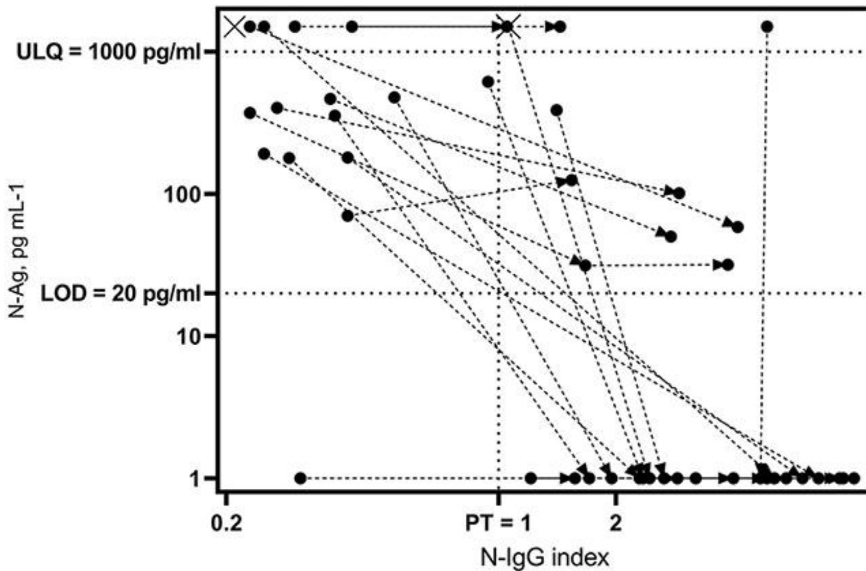
Fig. 4 Individual seroconversion patterns within 1st week after admission
