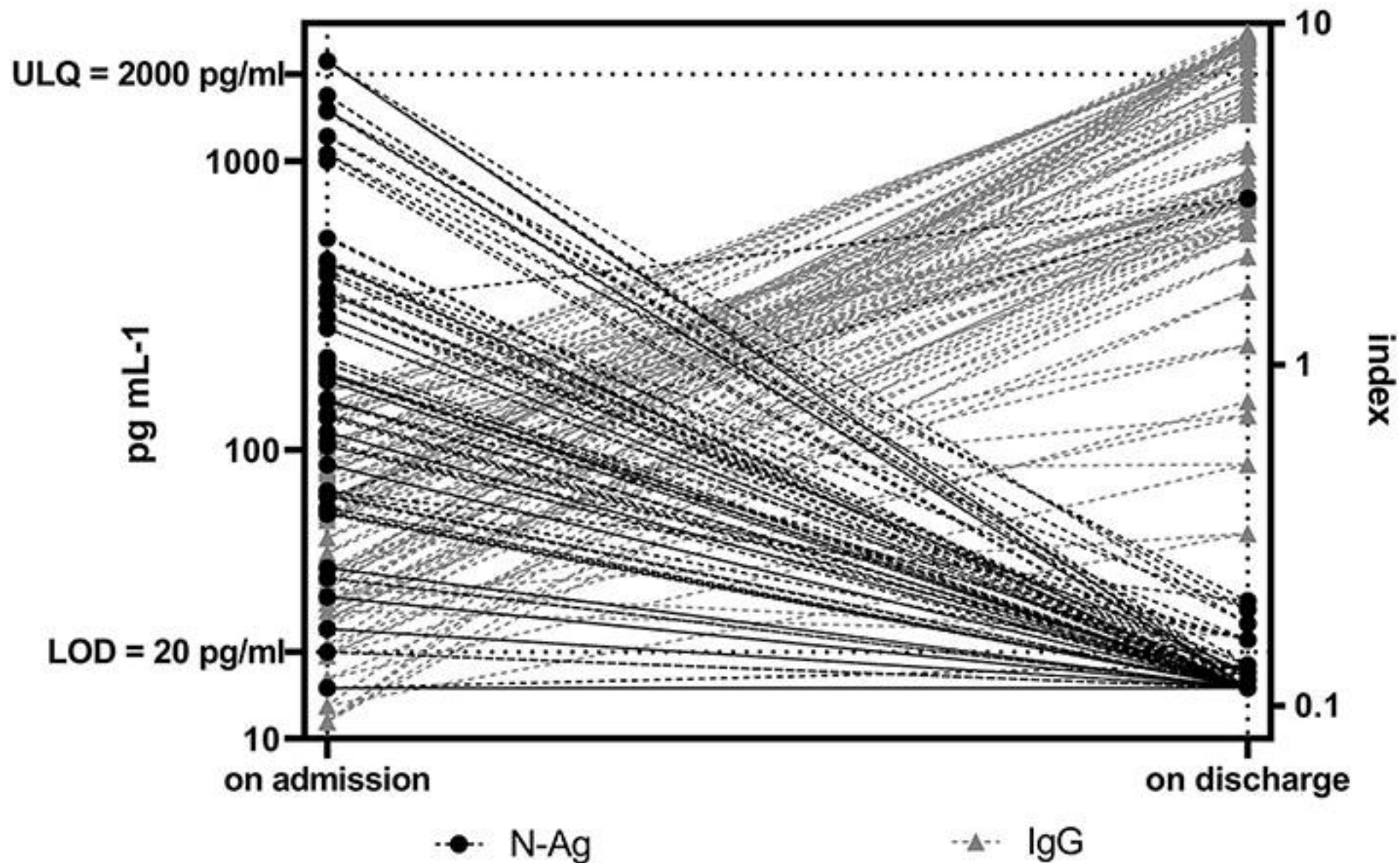
Fig. 2b Kinetics of N-Ag and IgG antibodies against N-Ag in patients seronegative on admission
