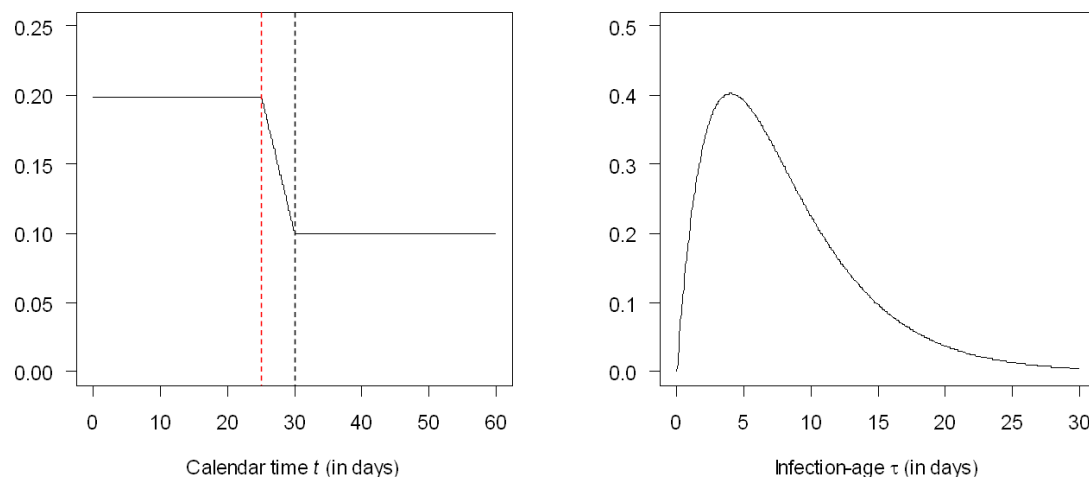
Figure 1: Components of the transmission rate \beta . The left panel shows the three phases of the pandemic: before lockdown at t = 25 (days), installation of lockdown (from t = 25 to t = 30 , between vertical dotted lines) and control of the disease ( t > 30 ). The right panel shows the transmission rate as a function of the infection age \tau .
