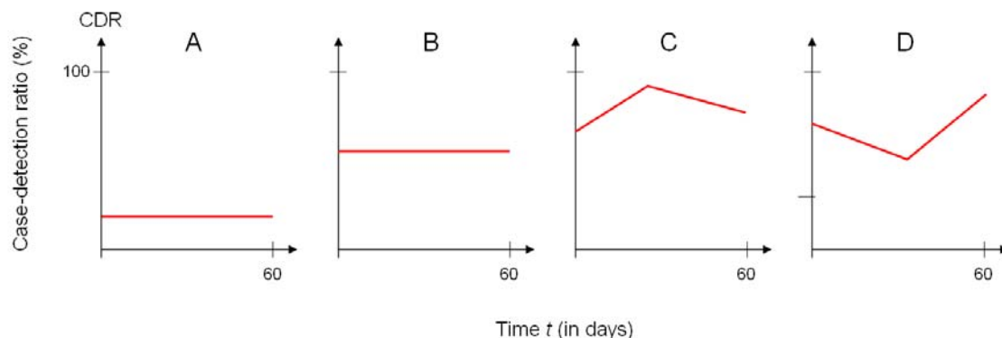
Figure 2: Scenarios of the time course of the case-detection ratio (CDR) during the pandemic.
