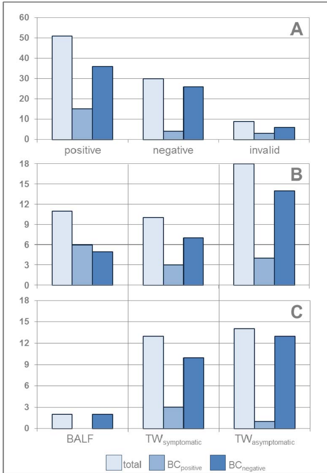
104 Figure 2: Specificity and sensitivity of SARS-CoV-2 antigen detection in PCR tested 105 specimen. (A) Analysis of the complete test cohort (n=90), consisting of PCR positive 106 (n=51), PCR negative (n=30) and PCR invalid samples (n=9), reveals an overall sensitivity of
