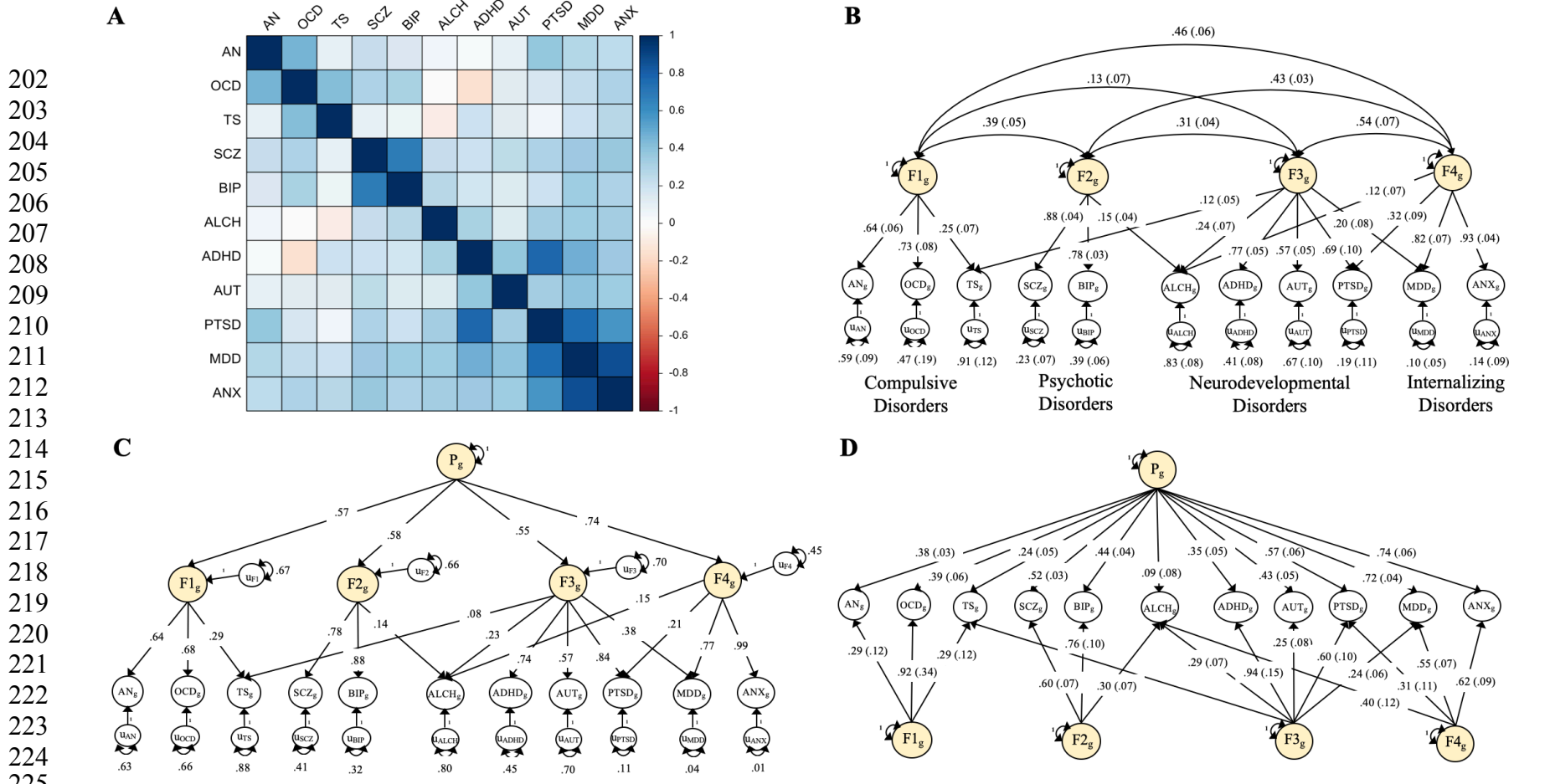
226 Figure 1. Multivariate Genetic Architecture of 11 Psychiatric Disorders. Panel A: Genetic correlations estimated using LDSC. Panel B: Standardized results 227 for the correlated factors. Panel C: Standardized results from the hierarchical factor model. Panel D: Standardized results from the bifactor model. The genetic 228 components of disorders and common genetic factors of disorders are inferred variables that are represented as circles. Regression relationships between 229 variables are depicted as one-headed arrows pointing from the independent variables to the dependent variables. Covariance relationships between 230 variables are represented as two-headed arrows linking the variables. (Residual) variances of a variable are represented as a two-headed arrow connecting the variable to itself; 231 for simplicity residuals of the indicators are not depicted for the bifactor model. ADHD = attention-deficit/hyperactivity disorder; OCD = obsessive-compulsive 232 disorder; TS = Tourette syndrome; PTSD = post-traumatic stress disorder; AN = anorexia nervosa; AUT = autism spectrum disorder; ALCH = problematic 233 alcohol use; ANX = anxiety; MDD = major depressive disorder; BIP = bipolar disorder; SCZ = schizophrenia.
