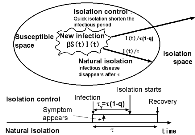
Fig.8 Concept of natural isolation in SIR model and isolation time control proposed in this work.
