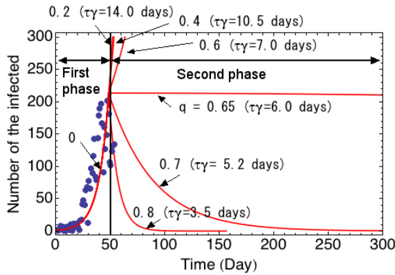
Fig. 9 Temporal evolution of the number of the infected for various isolation time control parameters q without any outing restriction c=0 . ( \tau_\gamma = \tau(1-q) and \tau = 17.54 days). Red lines are for \gamma=0.057 ( R_0=2.9 ).
