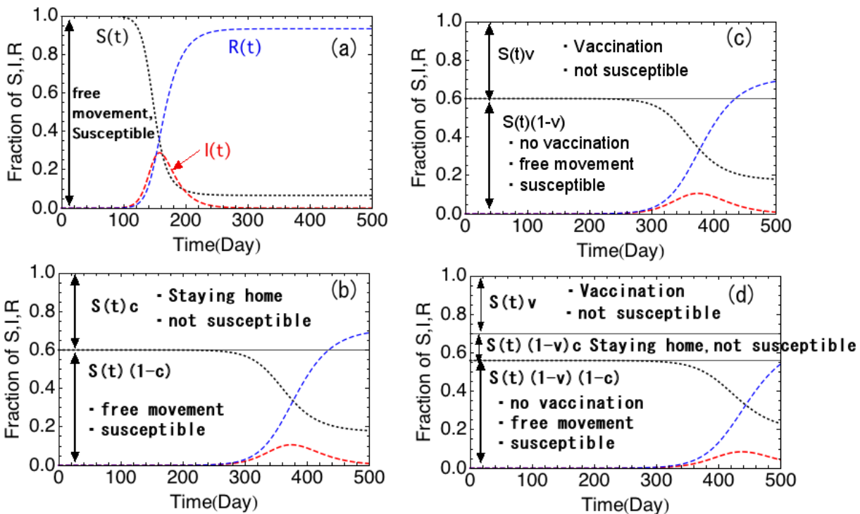
Fig. 4 The schematic SIR curves with the outing restriction and vaccination ratios. (a) No outing restriction, (b) Outing restriction alone with c=0.4 , (c) Vaccination alone with v=0.4 , and (d) vaccination ratio of v=0.3 and outing restriction ratio of c=0.2 .
