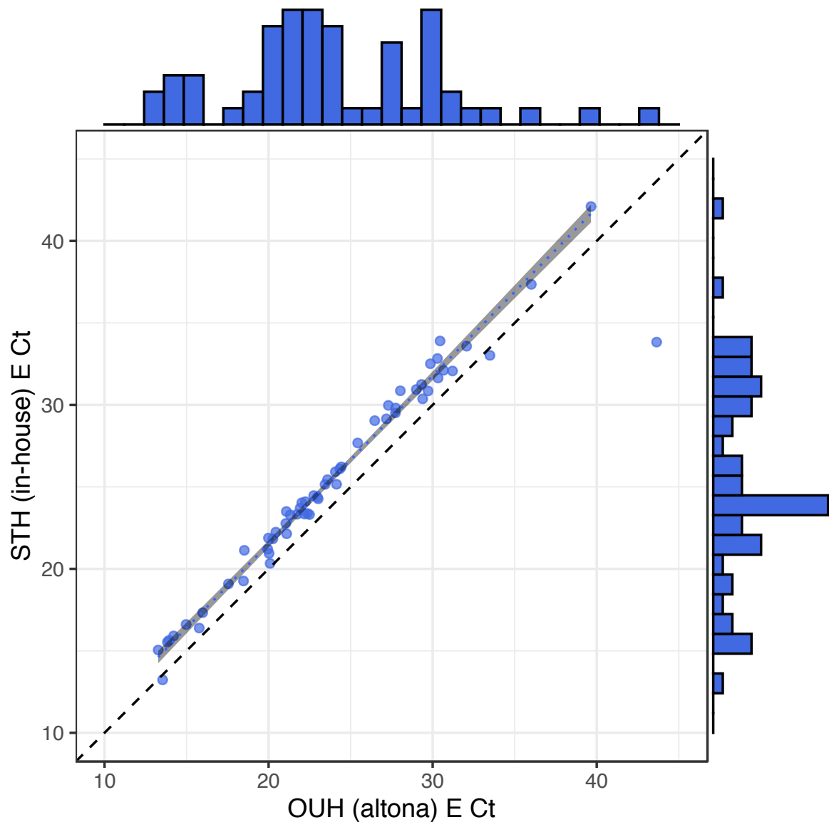
Figure S1 Comparison of E gene Ct values for 60 SARS-CoV-2 positive cross-site replicates between OUH and STH. Ct values at OUH were approximately one cycle lower than at STH, in part because of greater RNA input volume (10 \mu l at OUH vs 6 \mu l at STH). This line of best fit is plotted with shaded area representing 95% confidence intervals and excludes the single outlier.
