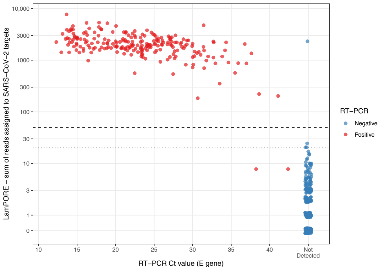
Figure 1 Total number of reads assigned to SARS-CoV-2 targets by LamPORE versus RT-PCR E gene Ct value. Dashed line is threshold for positive result ( \geq 50 reads), dotted line is threshold for inconclusive result ( \geq 20 reads). Invalid samples not plotted.
