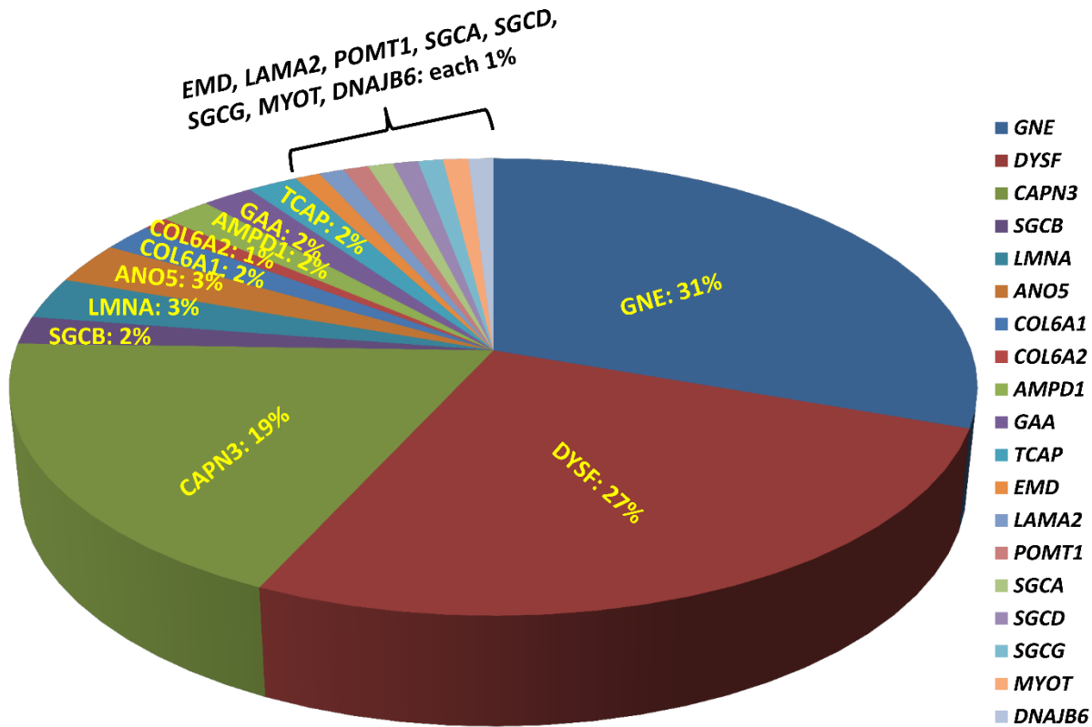
1011 FIGURE 1. Molecular diagnosis with different genetic myopathy subtypes. Molecular diagnosis 1012 using exome sequencing has been established in 49% of the patients with the majority having 1013 pathogenic variants identified in one of the following genes GNE (31%), DYSF (27%), CAPN3 1014 (19%), indicating that these genes are likely the major contributors to genetic myopathy-like 1015 phenotype.
