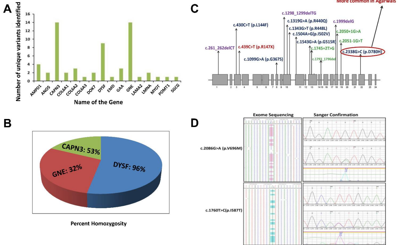
1027 FIGURE 2. Unique pathogenic variants and percent homozygosity identified in major 1028 myopathy genes. A) Number of unique pathogenic variants identified in major myopathy genes. B) 1029 The percentage of homozygosity observed in the major myopathy subtypes. Among the 3 major 1030 myopathy subtypes, 96% of the limb-girdle muscular dystrophy R2 (LGMDR2) patients caused by 1031 variants in DYSF gene were identified with homozygous variants. C) Mutation spectrum of CAPN3 1032 gene: CAPN3 variants identified in the current study are distributed throughout the gene. There is no 1033 specific mutation hot spot region but 3 variants are located in exon 10 indicating it as more unstable 1034 region prone to genetic variation. D) Two common variants in GNE gene: The two common variants 1035 in GNE gene were detected in exome sequencing with high confidence and also further confirmed by 1036 Sanger sequencing. Left side panel indicates the variants confirmation by exome sequencing. Right 1037 side panel indicates the variants confirmation by Sanger sequencing.
