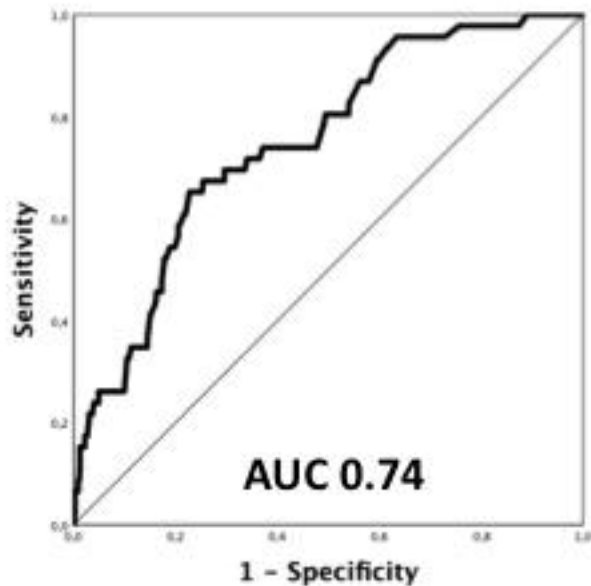
Validation dataset
