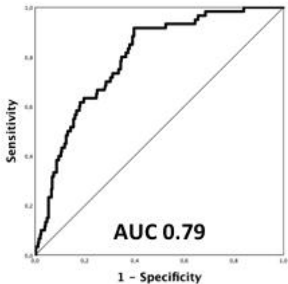
Developing dataset
