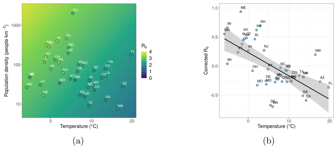
Figure 2: The relative importance of temperature and population density as drivers of pre-lockdown R_0 . (a.) Heatmap of the regression model R_0 predictions, with USA state-level R_0 point estimates overlaid. High population densities and low temperatures drive increases in SARS-CoV-2 R_0 . This is a 2D representation of the regression plane in fig. 1a, using the same colour-scale. (b.) Residuals from a linear regression of R_0 against \log_{10} -transformed population density (“Corrected R_0 ”), plotted against temperature. This illustrates that, when considering population density alone, R_0 is overestimated in cold states and underestimated in warm states. After accounting for population density, there is a significant effect of temperature upon R_0 (see table 1). In both figures, points are highlighted with standard two-letter state codes; MN and FL refer to Minnesota and Florida, respectively, and are referred to in the discussion.
