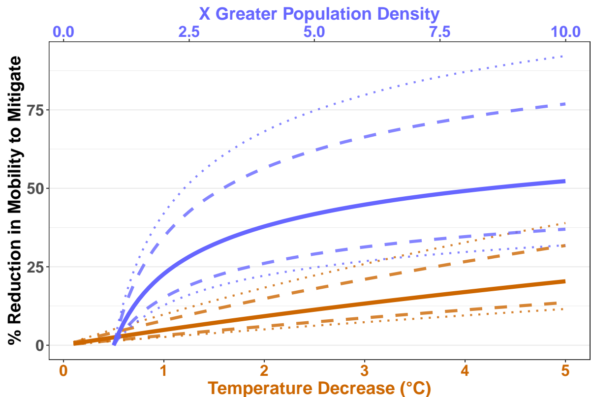
Figure 3: Average mobility reductions required to mitigate differences in population density and temperature. This figure shows the percent reduction in average mobility (measuring retail, recreation, grocery, pharmacy, and workplace trips) needed to compensate for a given temperature (brown) or population density (blue) driven increase in R_t . These calculations assume a ‘background’ R_0 of 1 and a baseline ‘background’ mobility (defined as ‘0’ by Google 36 ). Solid lines represent the median mobility reduction required, dashed and dotted lines the 75% and 90% posterior credibility intervals respectively.
