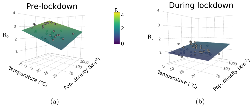
Figure 1: R_0 is affected by the environment, but the impact of lockdown is greater. (a.) R_0 plotted against temperature (averaged across the two weeks prior to the R_0 estimate) and \log_{10} -transformed population density (people per \text{km}^2 ) for each USA state (grey points). Surface shows the predicted R_0 from the regression model (table 1). Temperature has a negative effect on R_0 at state-level in the USA, whilst population density has a positive effect (table 1). (b.) The mean R_t for the two weeks following a state-wide stay-at-home mandate ( i.e. , during lockdown) plotted against average daily temperature for the same period and \log_{10} -transformed population density. The effects of temperature and population density are much weaker in the mobility-restricted data and R is reduced overall. The same colour scale, given in the centre of the figure, is used across both sub-plots.
