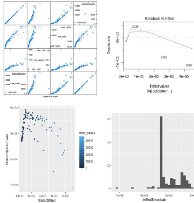
Figure 8. Scatter plot matrix and linear regression fit models
