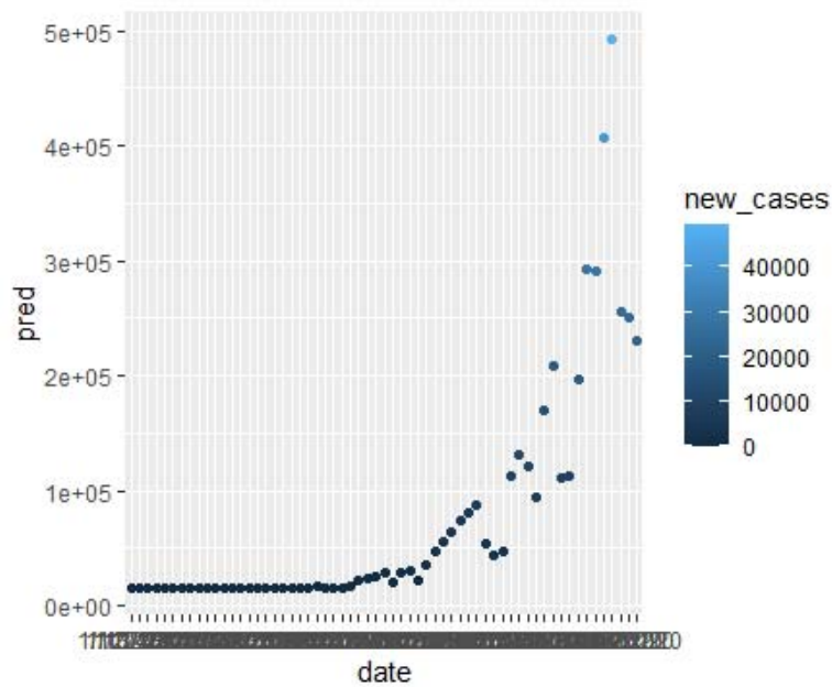
Figure 9 The prediction fit model
