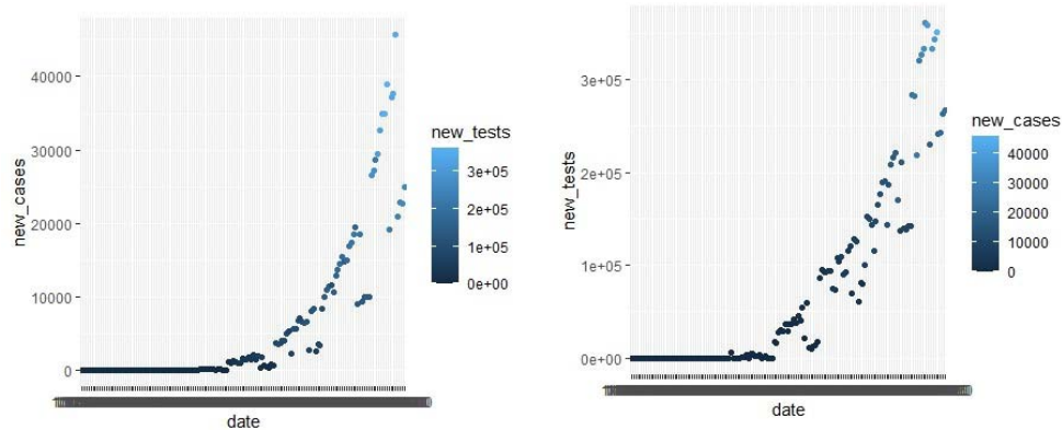
Figure 7 New cases and new tests for modeling
