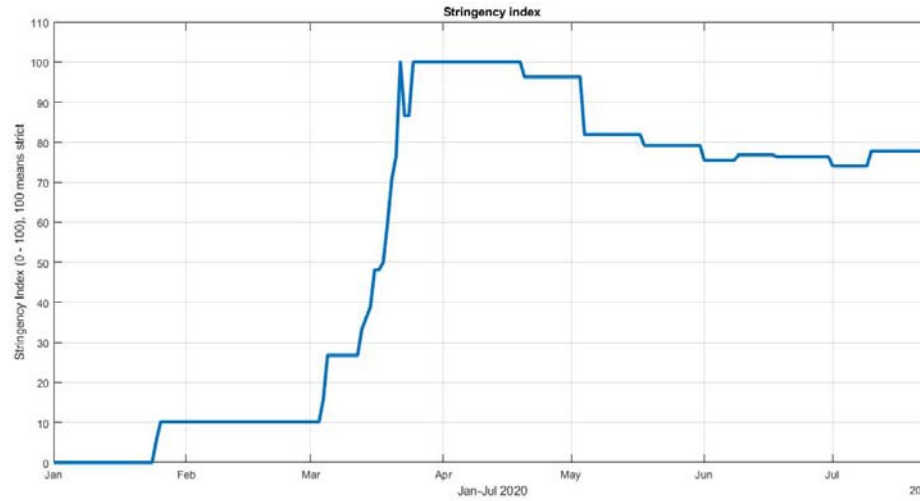
Figure 6 Stringency Index
