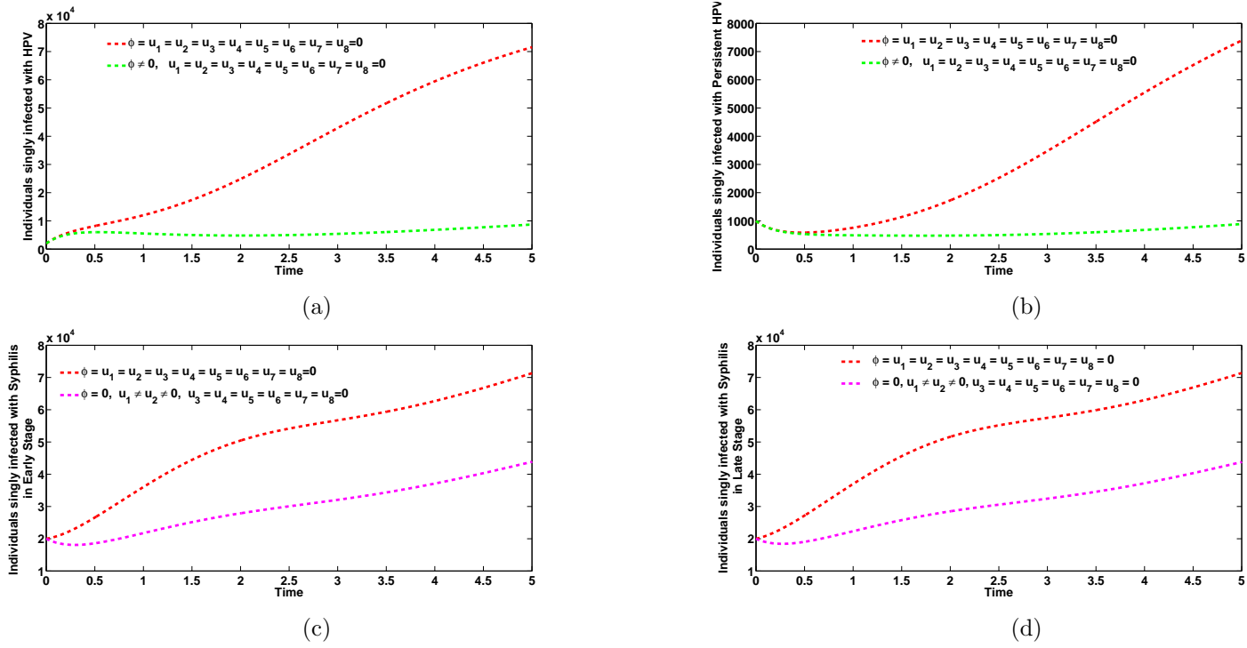
Figure 3: Plots of the total number of individuals singly infected with HPV and persistent HPV, respectively (Figures 3a and 3b) in the presence of optimal vaccination control only ( \phi \neq 0 ) and total number of individuals singly infected with syphilis in early and late stages of infection, respectively (Figures 3c and 3d) in the presence of treatment controls for singly infected only ( u_1 \neq u_2 \neq 0 ). Here, \beta_s = 7.0 , \beta_H = 2.0 . All other parameters as in Table 2
