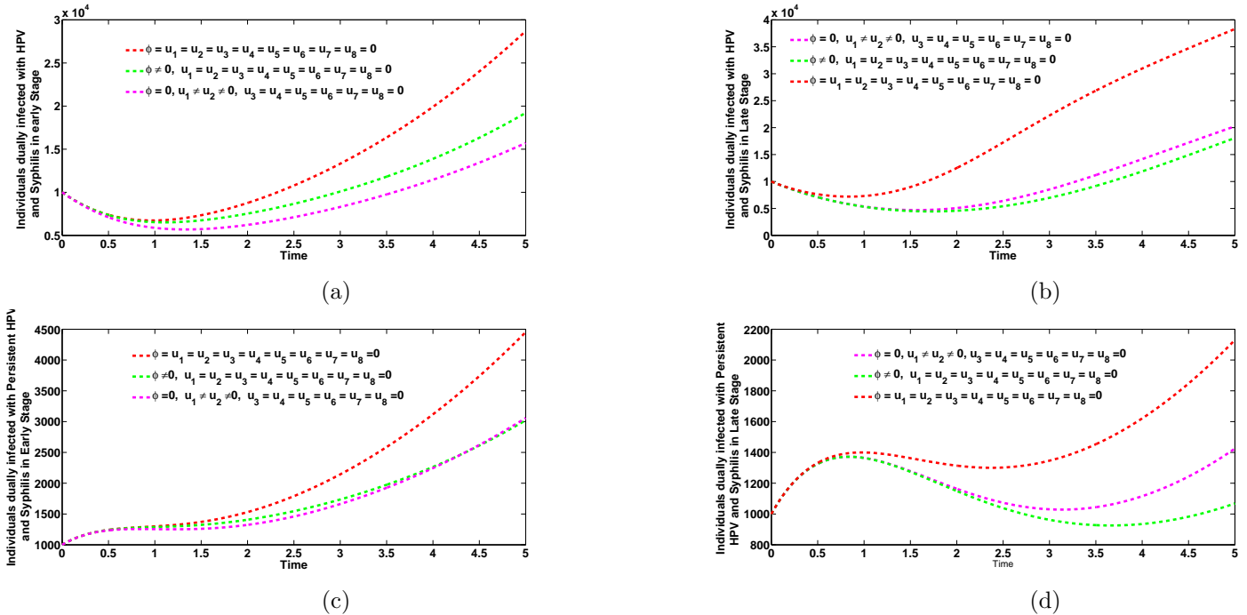
Figure 4: Plots of the co-infection cases for individuals dually infected with HPV and syphilis in early and late stages of infection, respectively (Figure 4a and 4b) and co-infection cases for individuals dually infected with persistent HPV and syphilis in early and late stages of infection, respectively (Figures 4c and 4d), when optimal vaccination control only strategy ( \phi \neq 0 ) and syphilis treatment controls for singly-infected ( u_1 \neq u_2 \neq 0 ) are administered. Here, \beta_s = 7.0 , \beta_H = 2.0 . All other parameters as in Table 2
