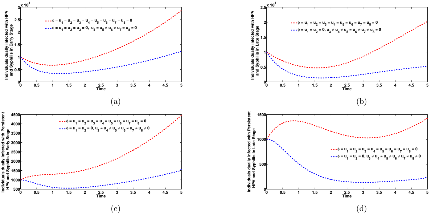
Figure 6: Plots of the co-infection cases for individuals dually infected with HPV and syphilis in early and late stages of infection, respectively (Figures 6(a) and 6b) as well as co-infection cases for individuals dually infected with persistent HPV and syphilis in early and late stages of infection, respectively (Figures 6c and 6d). Here, \beta_s = 7.0 , \beta_h = 2.0 , \phi = u_1 = u_2 = 0 , u_3 \neq u_4 \neq u_5 \neq u_6 \neq u_7 \neq u_8 \neq 0 . All other parameters as in Table 2
