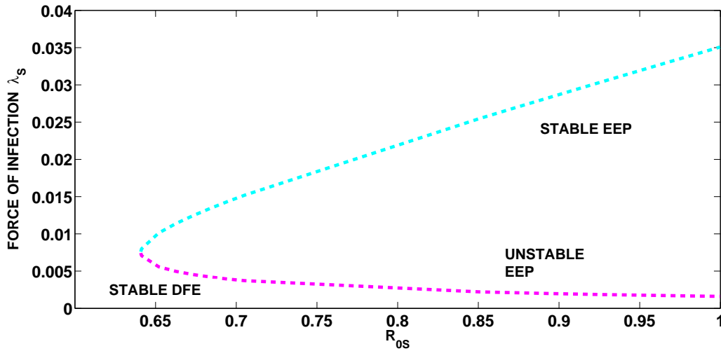
Figure 2: Bifurcation diagram for the syphilis-only sub-model (3). Parameter values used are: \beta_s = 3.0129 , \xi_s = 6.0 . All other parameters as in Table 2
