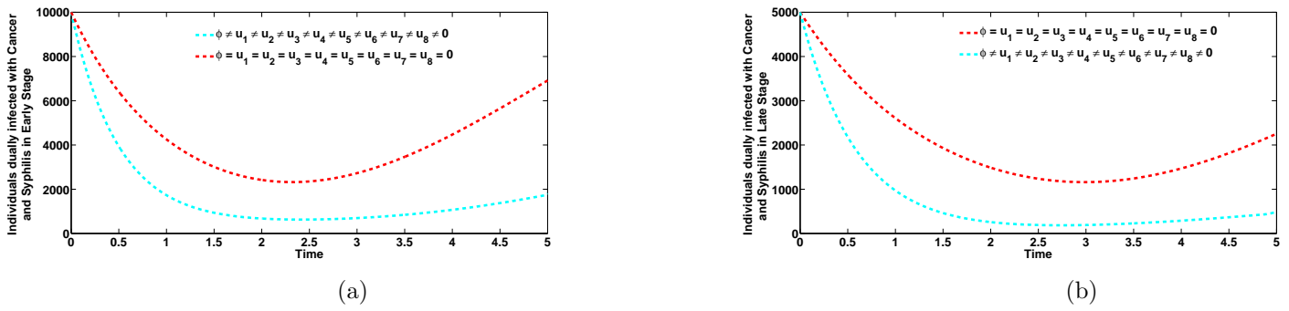
Figure 16: Plots of the co-infection cases for individuals dually infected anal cancer and syphilis in early and late stages of infection, respectively (Figures 16a and 16b), when there is universal control strategy and when there is no control administered. Here, \beta_s = 7.0 , \beta_H = 2.0 . All other parameters as in Table 2
