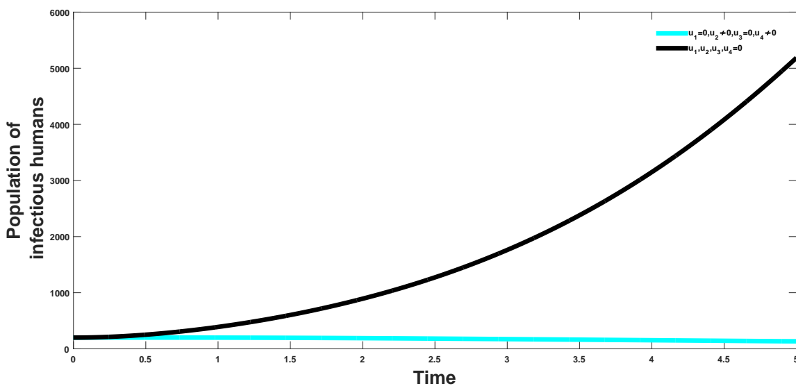
Figure 12: Combined effects of optimal controls u_2 and u_4 on the dynamics of the infected class
