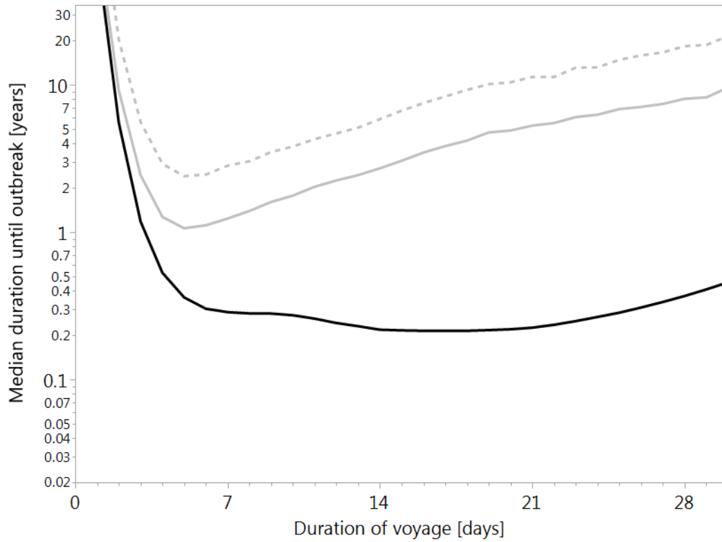
Figure 2: Median duration [log-scale in years] until a COVID-19 pandemic outbreak occurs in the destination country because of merchant ship crews taking shore leave. (a) 5, (b) 10, (c) 20 crew members per ship; 108 cargo ships arrive each week. In the country of origin, each member can pick up the infection at a rate of 0.00038 per day. Infections spread on board with an effective reproduction number R_{\text{eff}} of 3.0 and in NZ with R_{\text{eff}} of 2.5. Note that a voyage duration of 1 day is not applicable to NZ. Full black curves: no interventions are taken; full grey curves: all crew members are prevented from entering the country if one of them is PCR positive upon arrival; dotted grey curves: full set of interventions as outlined in Table 3. For each combination of crew size and voyage duration, 100 million voyages were simulated.
