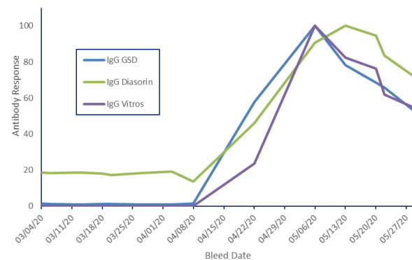
Figure 1. Levels of anti-SARS-CoV-2 IgG antibodies in a seroconversion panel as measured by three different assays. Each assay assigned arbitrary units to IgG levels so levels were normalized to a 100 point scale to allow comparison across assays.
