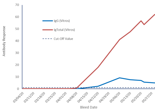
Figure 3. Anti-SARS-CoV-2 total immunoglobulins (Ig Total) and IgG measured in a SARS-CoV-2 seroconversion panel using Vitros ® kits. Values were expressed on an arbitrary scale relative specified by the manufacturer. For this assay, values \geq 1.0 were considered reactive (cut-off value) and values < 1.0 were considered non-reactive for SARS-CoV-2.
