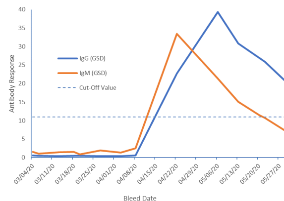
Figure 2. Anti-SARS-CoV-2 IgG and IgM antibodies measured in a SARS-CoV-2 seroconversion panel using Gold Standard SM Diagnostics (GSD) kits. Values are expressed on an arbitrary scale specified by the manufacturer. Values above 11 are considered reactive (cut-off value). Values between 9 and 11 were considered equivocal and values below 9 were considered non-reactive.
