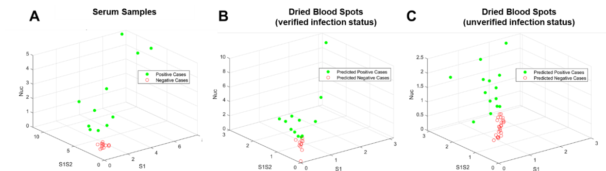
Figure 4. Visualization of testing data following machine learning-based analysis. (A) The GC-FP detection ratio data for all serum samples were plotted as a function of the three antigens S1, S1S2, and Nuc. These data were then used to train an SVM ML model, which was used to classify dried blood spot sample data from (B) subjects with verified COVID-19 infection status, and (C) subjects with unverified COVID-19 infection status.
