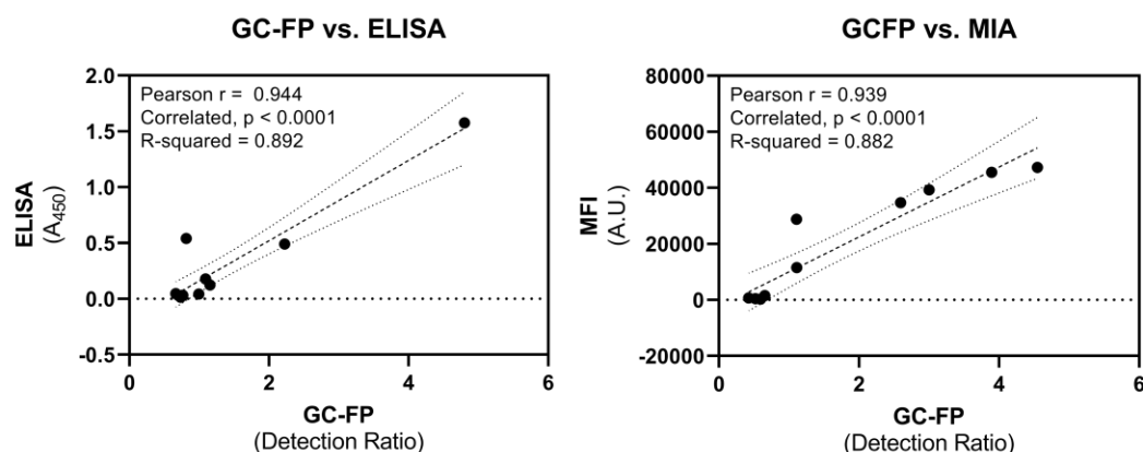
Figure 3. Correlation of ELISA and Luminex MIA results with GC-FP results for human serum samples. ELISA (450 nm absorbance values) for the COVID-19 nucleocapsid protein were compared to GC-FP detection ratio results for a subset of serum samples, while Luminex MIA results (MFI values) were compared to GC-FP detection ratio results for a second subset of samples. Pearson correlation coefficients ( r ) and R-squared values from correlation are shown, with associated p -values. Dashed lines indicate linear regression fit to the data, while dotted lines indicate the 95% confidence intervals for correlation analysis.
