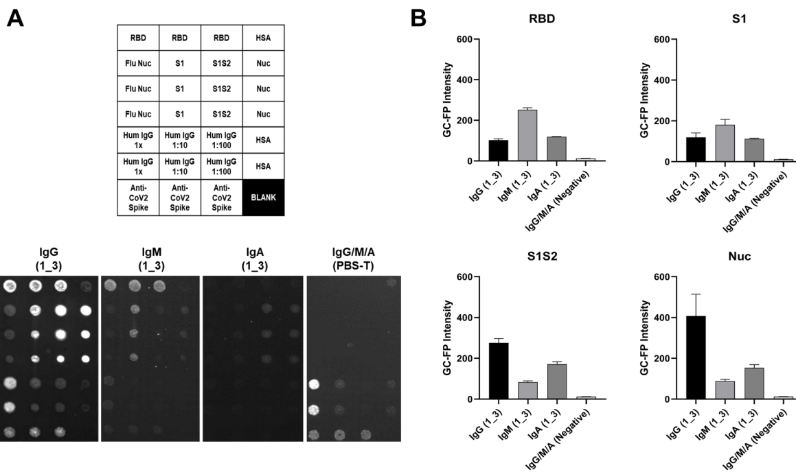
Figure 6. Serum sample 1_3 was tested on three separate v4 GC-FP biosensor chips that included RBD, S1, S1S2, and Nuc antigens. A fourth chip was processed using PBS-T as a negative control. The three chips tested with 1_3 serum were labeled with Alexa 647-tagged anti-human IgG, anti-human IgM, or anti-human IgA, while the negative control chip was labeled with a mixture of all three secondary antibodies. The mean GC-FP intensity ( n = 3 spots per chip) is shown, for each of the COVID-19 antigens.
