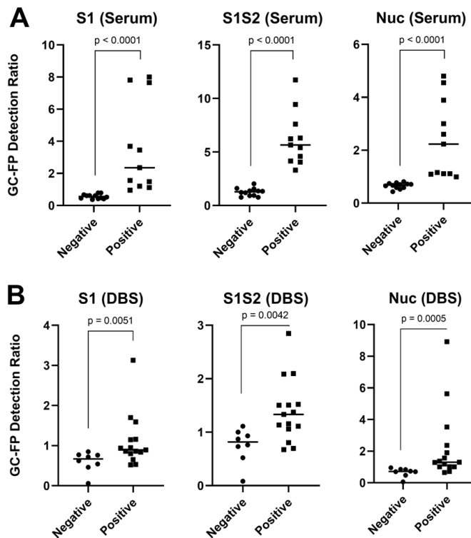
Figure 2. GC-FP assay results for serum (A) and dried blood spot (B) samples from subjects with verified positive COVID-19 infection (RT-PCR positive) or negative (including RT-PCR negative and subjects with no known exposure to COVID-19). GC-FP detection ratio is plotted for both positive and negative samples, for each individual antigen. A significant difference between the average positive and negative GC-FP detection ratios (horizontal line in each plot) was confirmed using the Mann-Whitney U-test, with corresponding p values shown in each plot.
