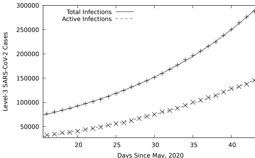
Figure 1: Level-3, best fits to SARS-CoV-2, infection data (16th of June to the 13th of July, 2020).
