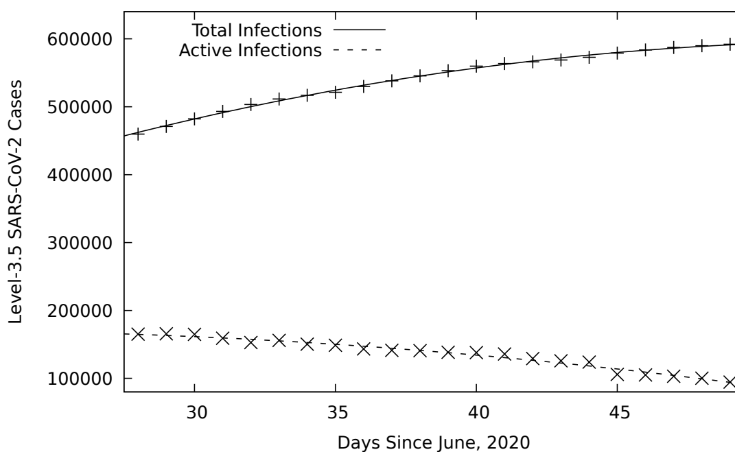
Figure 2: Level-3.5, best fits to SARS-CoV-2, infection data (28th of July to the 18th of August, 2020).
