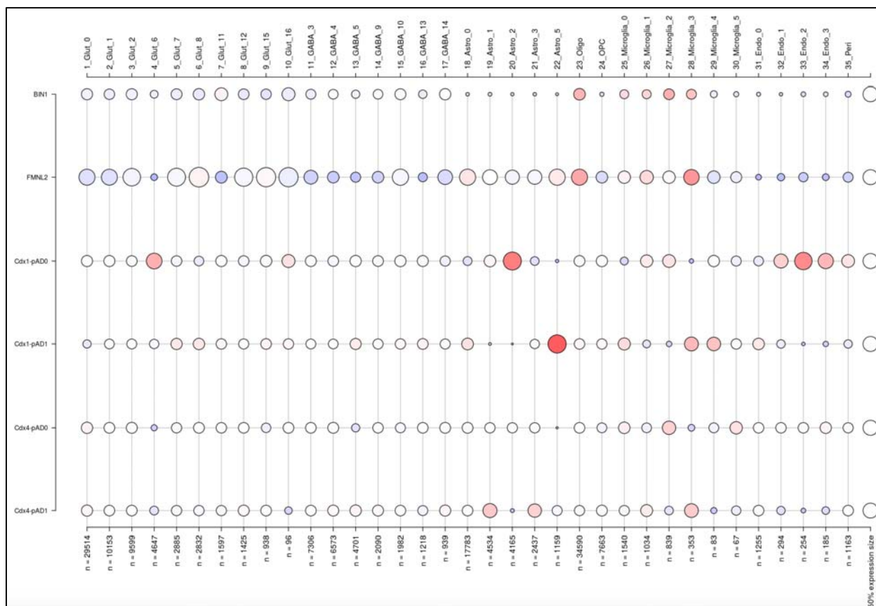
Figure 2. Single cell expression from ROSMAP dorsolateral frontal cortex. Expression levels of genes and participant diagnosis categories within cell type specific clusters. Cell type specific clusters: Cdx1-pAD0: non-impaired individuals without pathologic criteria for AD by the NIA Reagan scale, (2) Cdx1-pAD1: cognitively non-impaired individuals fulfilling pathologic criteria for AD, (3) Cdx4-pAD0: individuals with dementia who do not fulfill pathologic criteria for AD, and (4) Cdx4-pAD1: individuals with dementia who also fulfilling pathologic criteria for AD.
