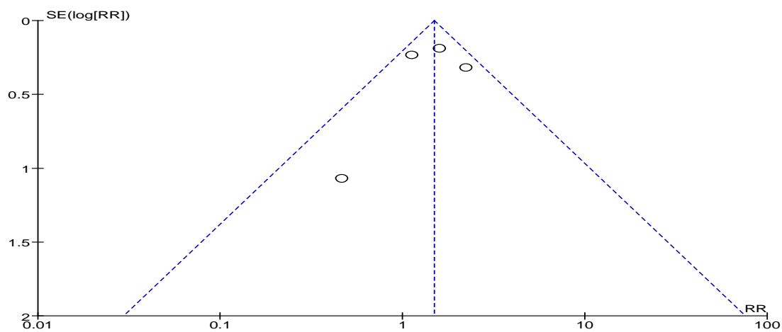
Figure 5. Funnel plot
