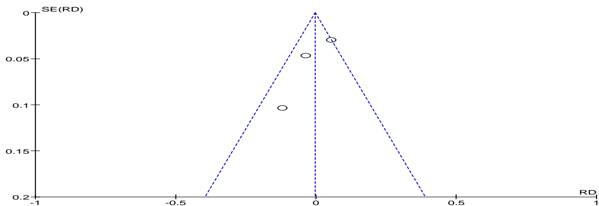
Figure 8. Funnel plot
