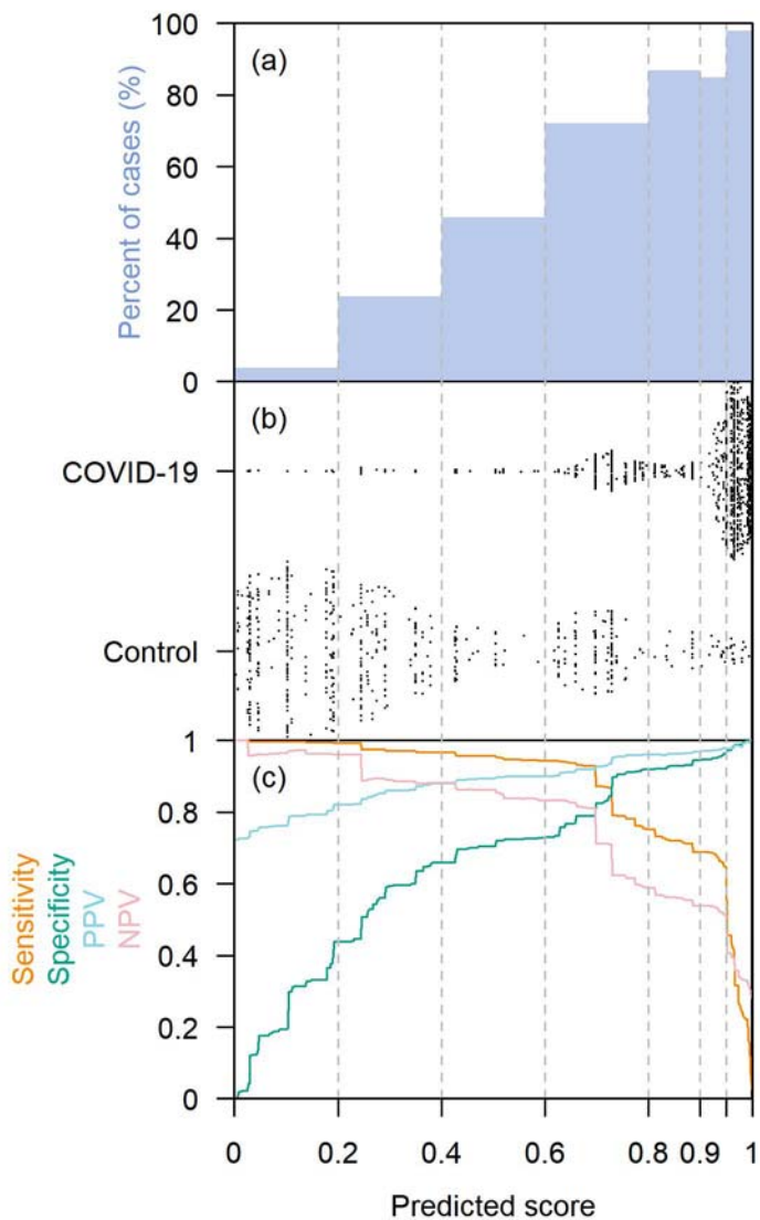
Figure 4: Comparisons of predicted risk to observations, (a) shows bars with the height indicating the percentage of cases in respective intervals of predicted risk. (b) plots the predicted risk grouped by case or control. (c) traces the calculated in-sample sensitivity, specificity, PPV and NPV for a grid of predicted risks as cutoffs spaced at 0.001 from 0 to 1.
