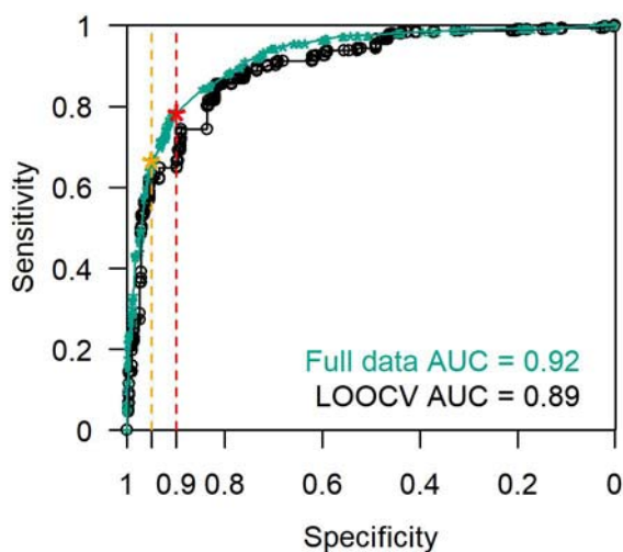
Figure 3: ROC curve with LOOCV. AUC = 0.89. Using full data, AUC = 0.92. With a minimum specification threshold at 0.95 and 0.9, the cutoff points are found at 0.92 and 0.74 respectively as indicated by the orange and red stars on the curve.
