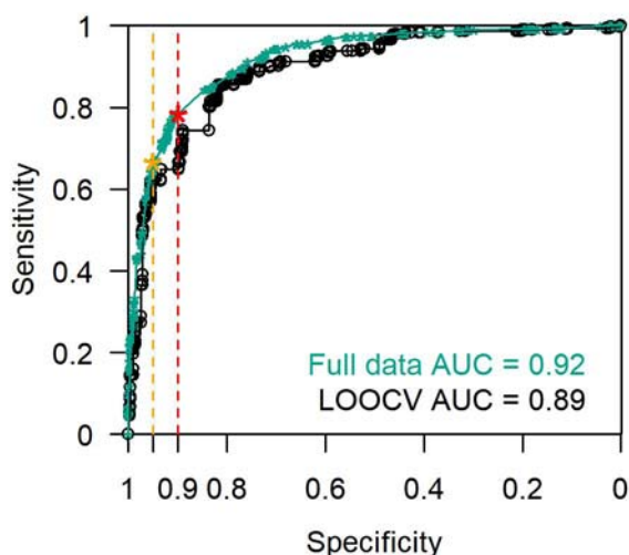
Figure 3: ROC curve with LOOCV. AUC = 0.89. Using full data, AUC = 0.92. With a minimum specification threshold at 0.95 and 0.9, the cutoff points are found at 0.92 and 0.74 respectively as indicated by the orange and red stars on the curve.
