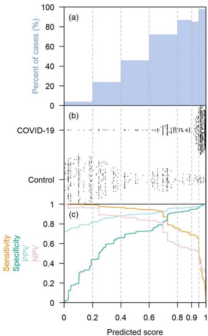
Figure 4: Comparisons of predicted risk to observations, (a) shows bars with the height indicating the percentage of cases in respective intervals of predicted risk. (b) plots the predicted risk grouped by case or control. (c) traces the calculated in-sample sensitivity, specificity, PPV and NPV for a grid of predicted risks as cutoffs spaced at 0.001 from 0 to 1.
