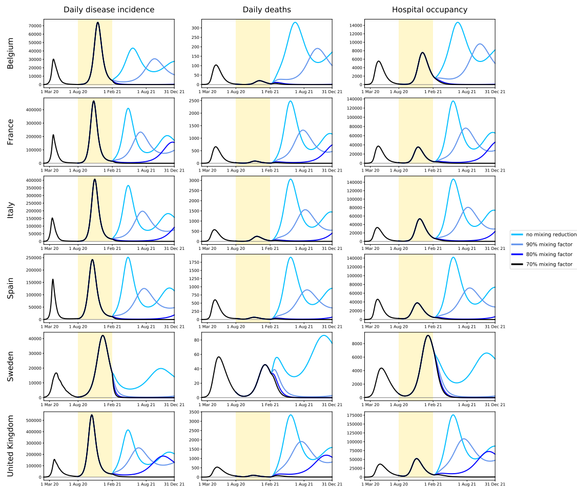
Figure 8. Predicted COVID-19 incidence, mortality and hospital occupancy over time with short-lived post-infection immunity and applying mild mixing reductions after the optimised phase
