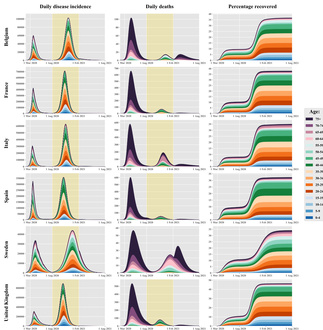
Figure 5. Age-specific profile of disease incidence, COVID-19-related deaths and proportion recovered over time optimised for life-years lost (6-month mitigation by age)
