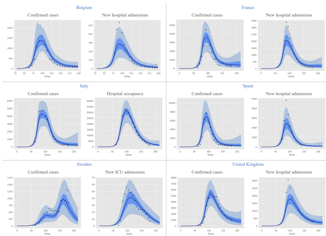
Figure 2. Model projections compared against local data
