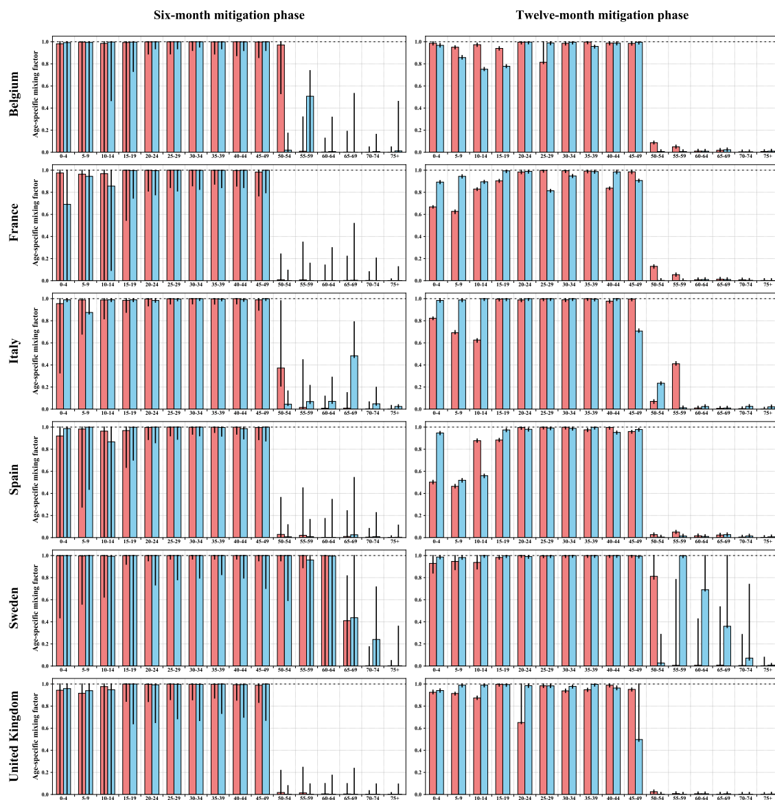
Figure 3. Optimal mixing pattern with contact mitigation by age
