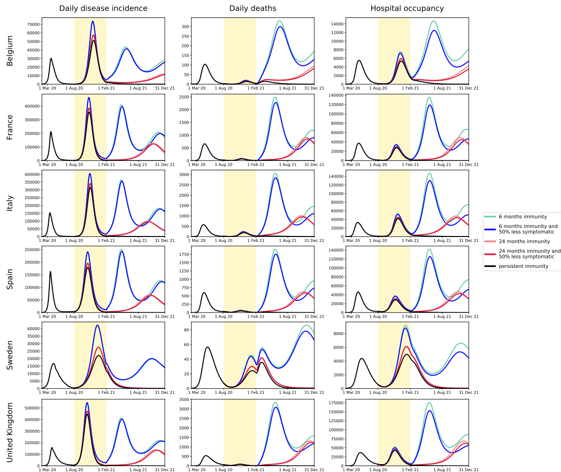
Figure 7. Predicted COVID-19 incidence, mortality and hospital occupancy over time under various assumptions of waning immunity
