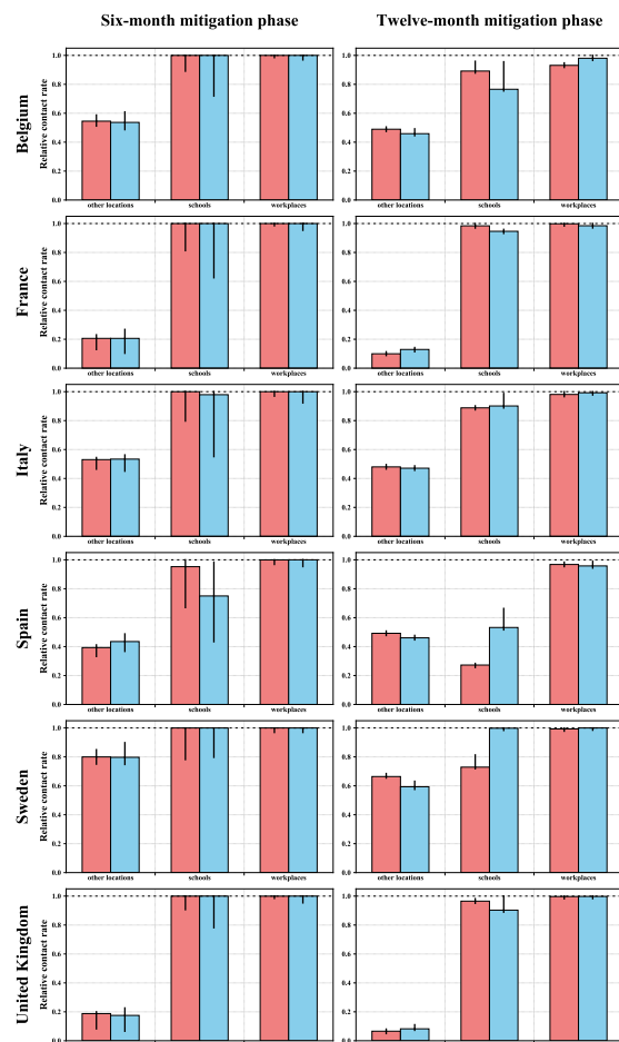
Figure 4. Optimal mixing pattern with contact mitigation by location
