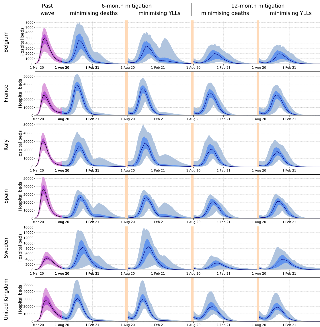
Figure 6. Predicted hospital occupancy during the past wave compared to a second wave that would achieve herd immunity (optimised mitigation by age, assuming persistent immunity)
