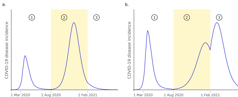
Figure 1. Illustration of the three simulation phases
