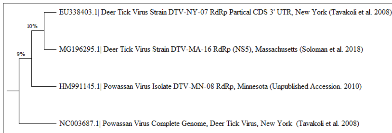
Figure 3. Evolutionary Relationships of Powassan Virus Lineage II, DTV in the United States. 2,3 The evolutionary history was inferred using the UPGMA method [14]. The optimal tree with the sum of branch length = 0.19223306 is shown. The tree is drawn to scale, with branch lengths in the same units as those of the evolutionary distances used to infer the phylogenetic tree. The evolutionary distances were computed using the Maximum Composite Likelihood method [15] and are in the units of the number of base substitutions per site. This analysis involved 4 nucleotide sequences accessed through GenBank. Codon positions included were 1st+2nd+3rd+Noncoding. All ambiguous positions were removed for each sequence pair (pairwise deletion option). There was a total of 10840 positions in the final dataset. Evolutionary analyses were conducted in MEGA X [16]
