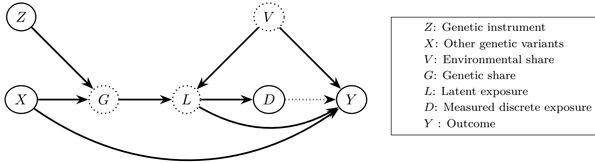
Figure 2: The framework proposed in Section 2 summarised in a directed acyclic graph. Dotted circles represent latent variables and complete circles represent observed variables.
