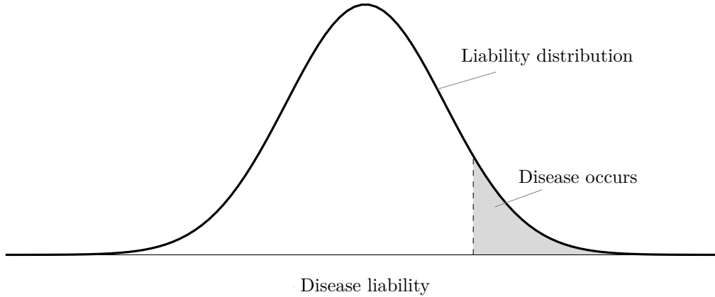
Figure 1: In the Falconer framework, liability to a disease is assumed to follow a smooth (often normal) distribution. The disease occurs at the tail of the distribution, with the grey region representing prevalence in the population.
