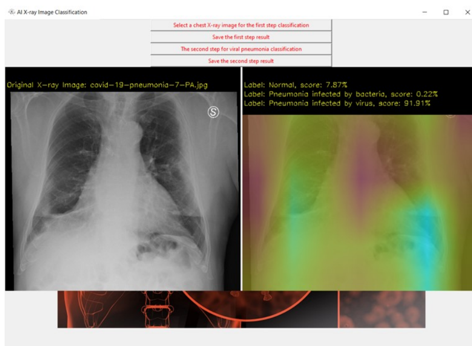
a) Results from step.1. Left image shows the original X-ray data, Right image shows the possibility of 3 different cases (normal, infected by bacteria, infected by virus) and brighter color shows which part has the potential infection problem.
