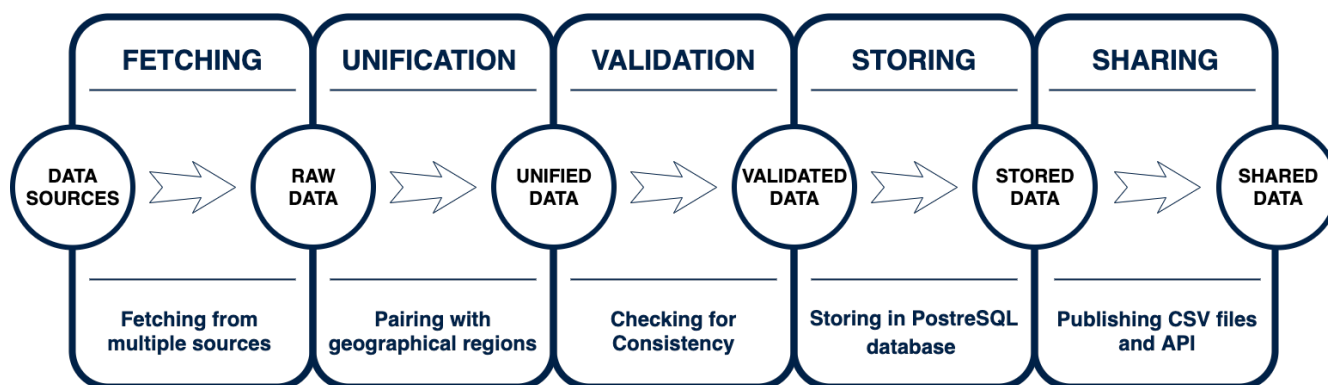
Figure 3. System architecture for OxCOVID19 Database.
