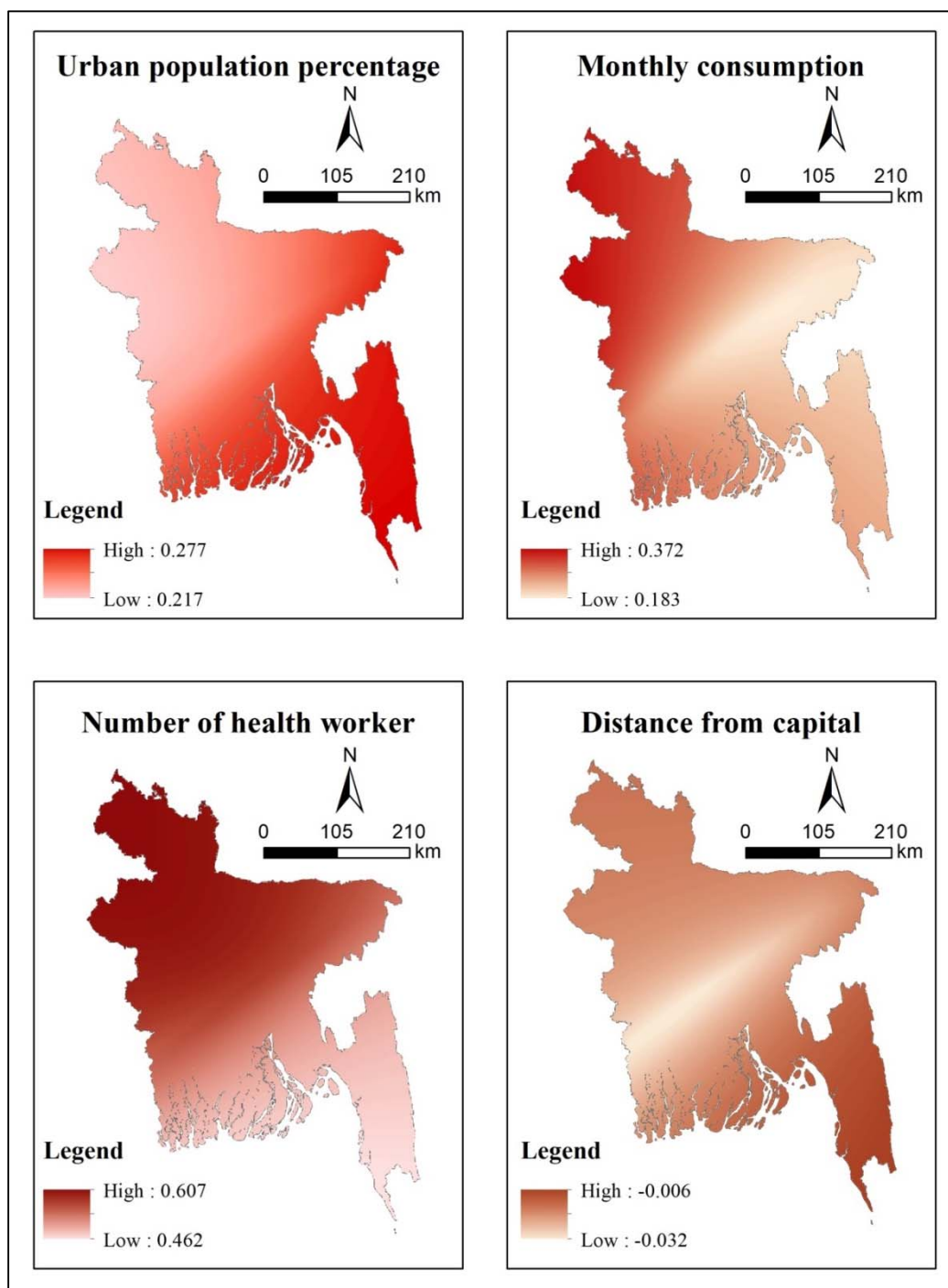
Figure 3: Spatial distribution of the coefficient values of urban population percentage, monthly consumption, number of health workers, and distance from the capital in describing COVID-19 incidence rates using GWR model
