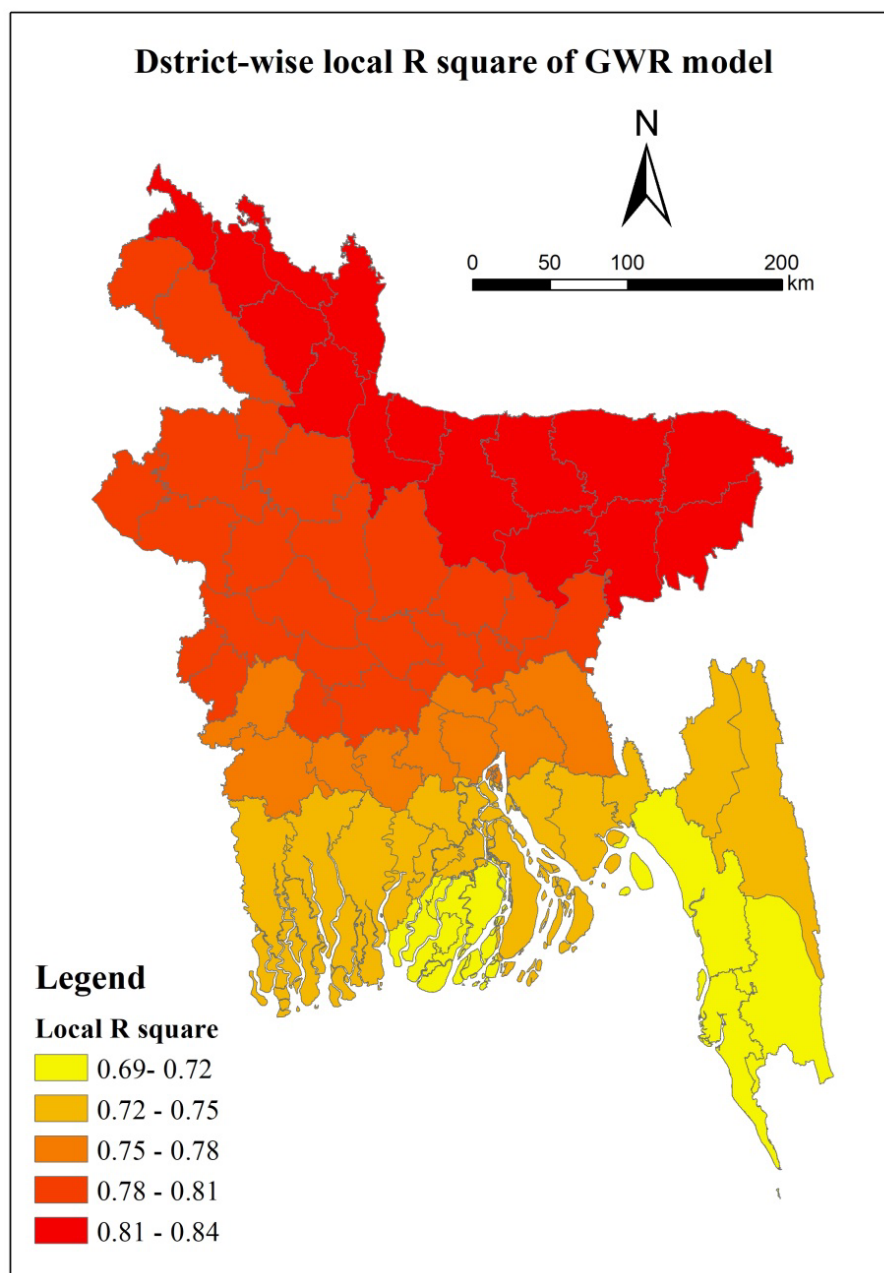
Figure 4: Spatial distribution of the local R^2 values of GWR model
