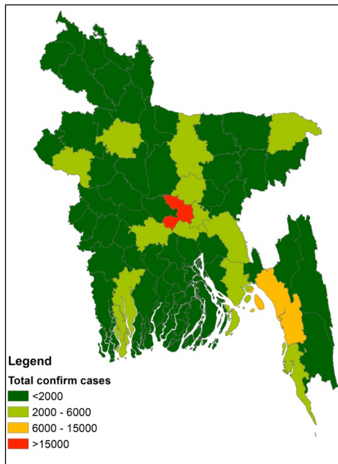
Figure 1: Number of confirmed COVID-19 cases by district
