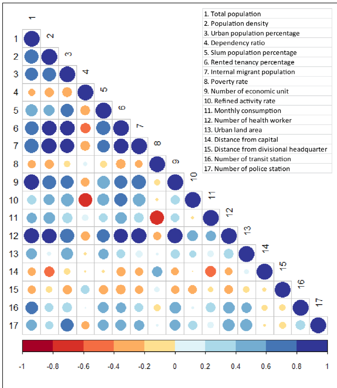
Figure 2: Results of the correlation analysis
