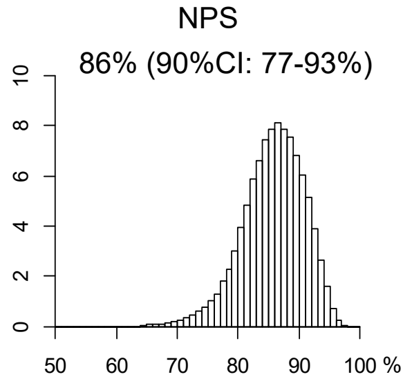
Figure 2 (a) sensitivity
