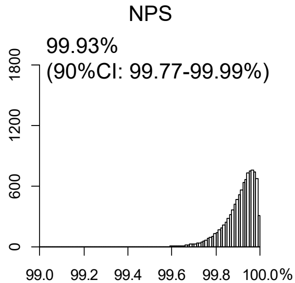
(b) specificity
