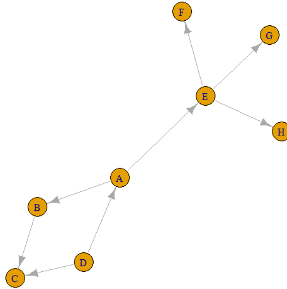
Figure 2. A contact graph
