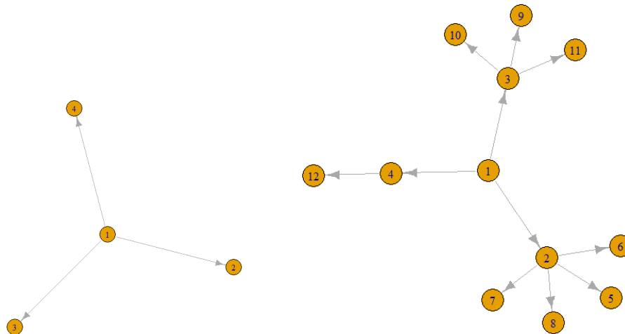
Figure 6. The first (on the left) and second stages (on the right) of COVID-19 transmission graphs
