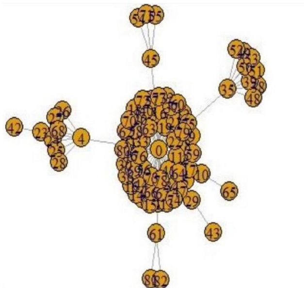
Figure 7: Network structure of COVID-19 infections in India until March 13, 2020 [33]
