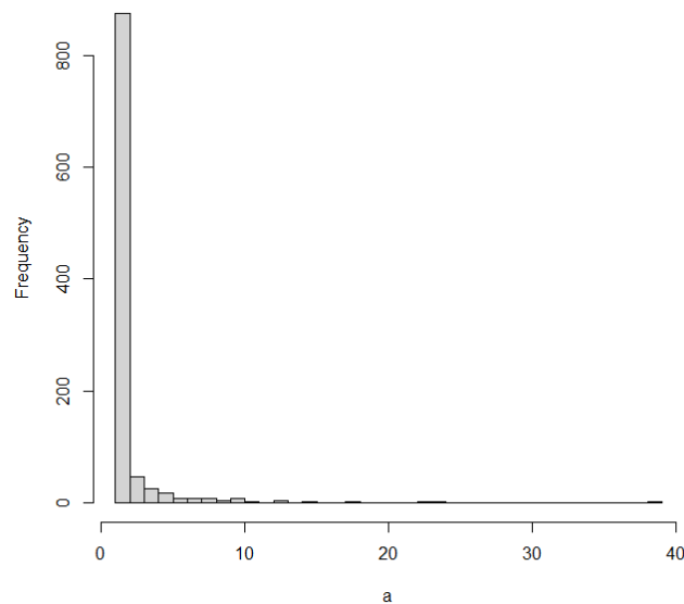
Figure 1. Histogram of a simulated discrete Pareto distribution
