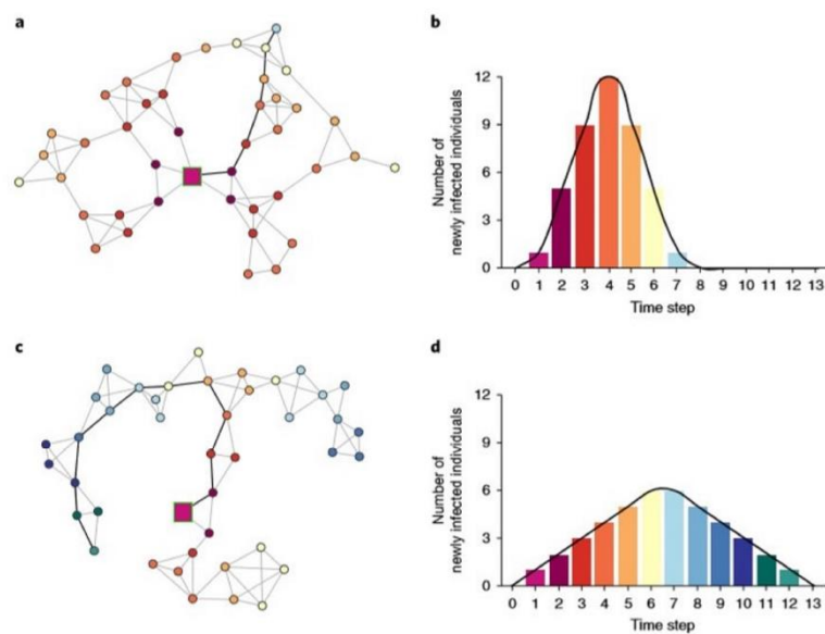
Figure 4. Two example networks. a–c with the same number of nodes and ties [31]
