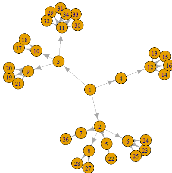
Figure 5. COVID-19 transmission graph using simulated discrete Pareto distribution values
