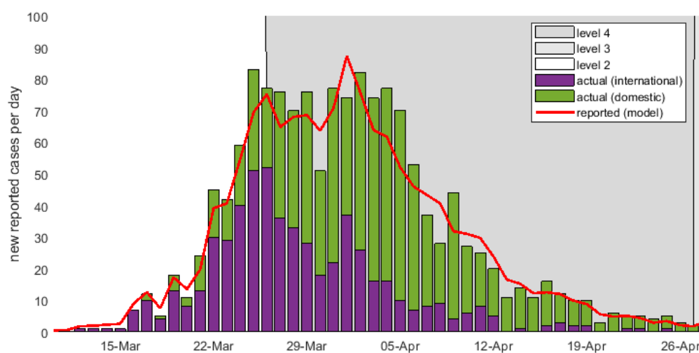
Figure 1: Simulated and actual daily numbers of new local and imported cases (confirmed and probable) in New Zealand prior to and during Alert Level 4. The values of R_{eff} that gave the best model fit to the data, evaluated using a least squares approach, were R_{eff} = 1.8 prior to lockdown and R_{eff} = 0.35 in Alert Level 4.
