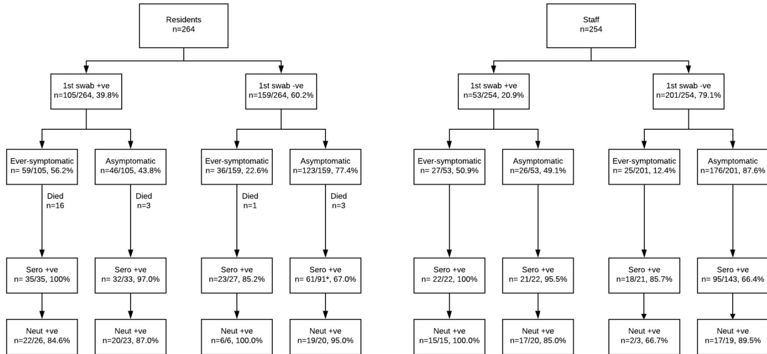
Figure 1. Flow diagram of residents and staff in 6 London care homes experiencing a COVID-19 outbreak during the pandemic who consented to follow-up testing including blood sampling for SARS-CoV-2 antibodies four to six weeks later. ‘Ever-symptomatic’ indicates that symptoms were experienced at some point during the follow-up period.
