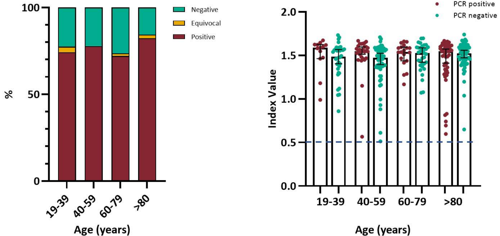
Figure 3. Age group analysis native viral antigen lysate assay. Left panel: Seroconversion percentage by age group for whole cohort, N=394. Right panel: Native viral antigen assay index value for seropositive individuals by initial RT-PCR status and age group, N=307. Bars indicate median and 95% confidence interval. Dashed line indicates assay positive cut-off. Statistical analysis using Chi square test of proportion and Kruskal-Wallis with Dunn's multiple comparisons test, no significant difference.
