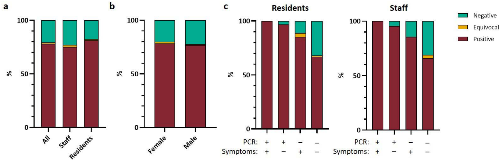
Figure 2. Proportion of indicated study populations with positive (maroon), equivocal (yellow) or negative (green) native viral antigen lysate assay. a) Seroconversion for all cohort and staff and resident sub groups. b) Seroconversion by sex for whole cohort. c) Seroconversion by acute RT-PCR result and presence of symptoms for residents and staff. All N = 394; Staff N= 208; Residents N= 186.
