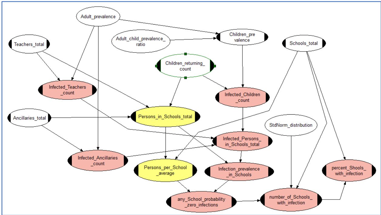
207 Figure 1. Bayesian Belief Network to calculate schools COVID-10 infection hazard with prevalence 208 represented by a single random variable. In order to account for regional variations of prevalence later 209 BBN modelling introduced a range of random variable values for prevalence in different geographical 210 areas as depicted in Figure 3. Plain white nodes carry input variable uncertainty distributions, white 211 nodes with handles represent fixed (constant) input values. Yellow nodes are intermediate functional (i.e. 212 calculational) nodes. Pink nodes compute the required output variable probability distributions; some 213 these are also intermediate calculation steps, feeding uncertainty distributions into other output nodes.
