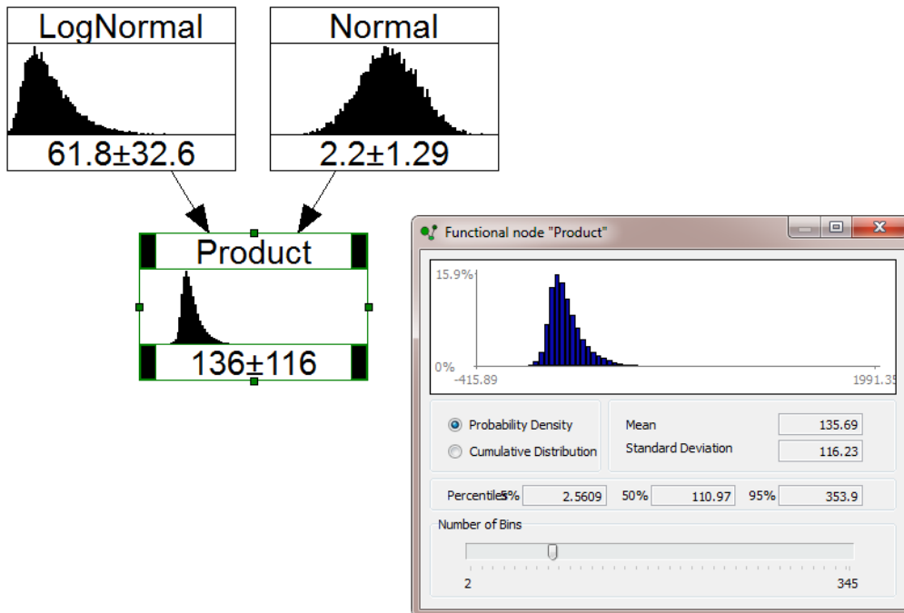
742 743 744 Figure A1. Simple UNINET model showing how variable uncertainty distributions can be 745 represented by probability nodes (e.g. LogNormal, Normal) and calculations can be made with 746 functional nodes containing equations or formulae (e.g. node Product). For a set number of
