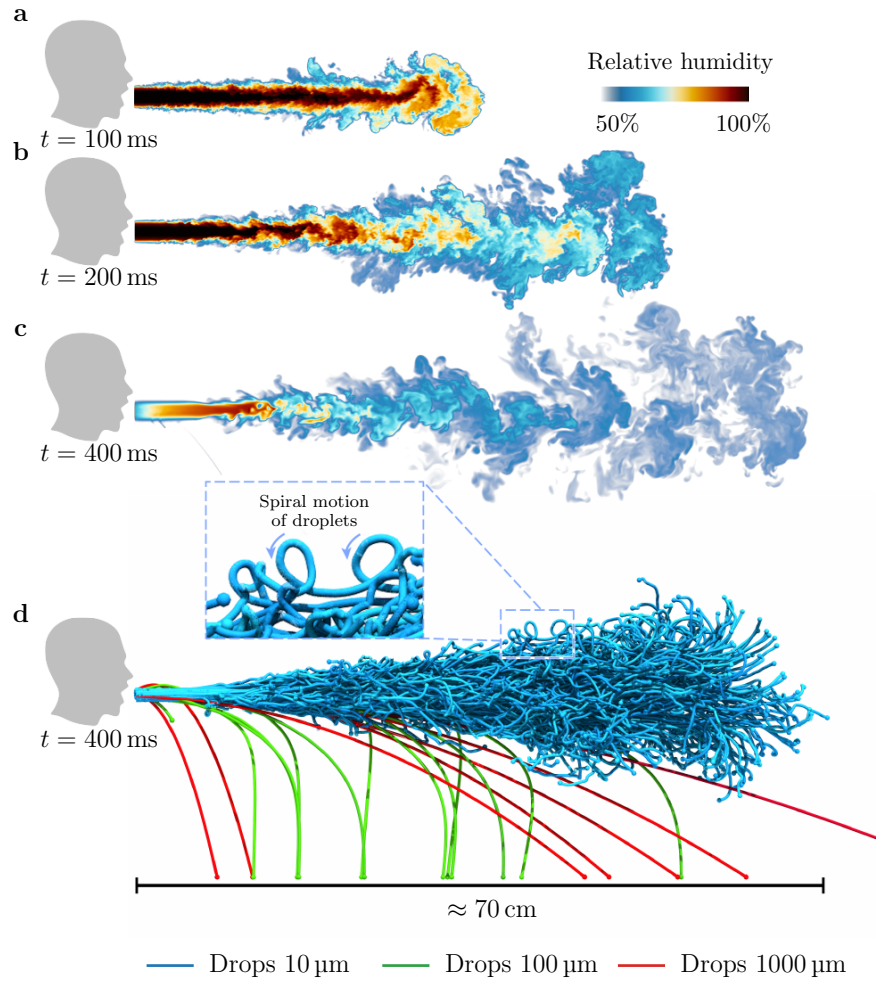
Figure 1: Visualisations of droplets in a heavy cough for RH = 50\% : a-d , Snapshots of the droplet-laden cough simulation. At time t = 100 ms, the cough contains hot air with high moisture content. The hot moist air propagates ( t \approx 200 ms) and dissipates ( t \approx 400 ms) into the ambient surroundings. At t \approx 400 ms, we show larger droplets falling out from the puff whereas smaller droplets remain protected and are carried along by the puff.
