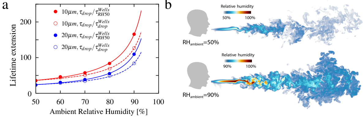
Figure 4: Lifetime ratio for 10 \mu\text{m} and 20 \mu\text{m} droplets: a , Extended lifetime as a function of relative humidity up to \text{RH} = 90\% . The curves in the figure are fitted according to the function y = a_1/(1 - x) + a_2 , where a_1 and a_2 are the fitting parameters. Visualisations of humid puff for ambient RH = 50% and 90% at time 600 ms: b , The humid puff maintains coherence for longer time and at much longer distances for larger ambient RH. Note the different humidity color scales for two shown cases.
