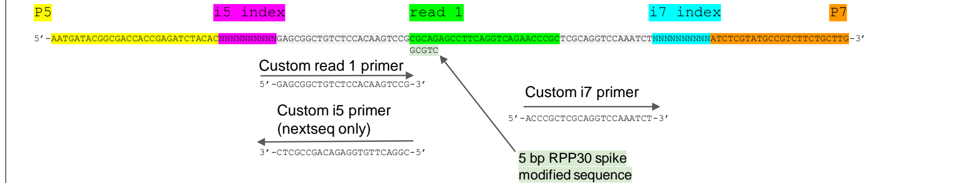
Figure S1. Sequencing library design. The amplicon designs are shown for the S2 (top) and RPP30 (bottom) amplicons. Amplicons were designed such that the i5 and i7 molecular indexes uniquely identify each sample. SwabSeq was designed to be compatible with all Illumina platforms.
