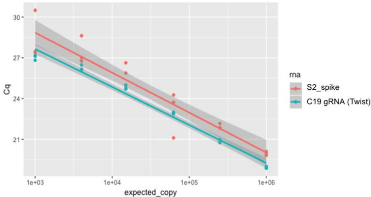
Figure S2. S2 primers show equivalent PCR efficiency when amplifying the COVID-19 amplicon and the synthetic S2 spike. Slope of PCR efficiency of the primers with either the S2_spike or the SARS-CoV-2 viral (labeled in green as C19gRNA) input are as follows: S2_spike slope = -6.68e-6 and C19gRNA(Twist Control) slope = -6.74e-6 . The slopes are expected to equivalent (parallel) if the primers do not show preferential amplification of the S2 spike RNA versus the C19gRNA. This shows that the S2 spike and C19gRNA have equivalent amplification efficiencies using the S2 primer pair. The bands represent 95% confidence intervals for predicted values, are non-overlapping due to different intercepts, and are not relevant for this analysis of slopes.
