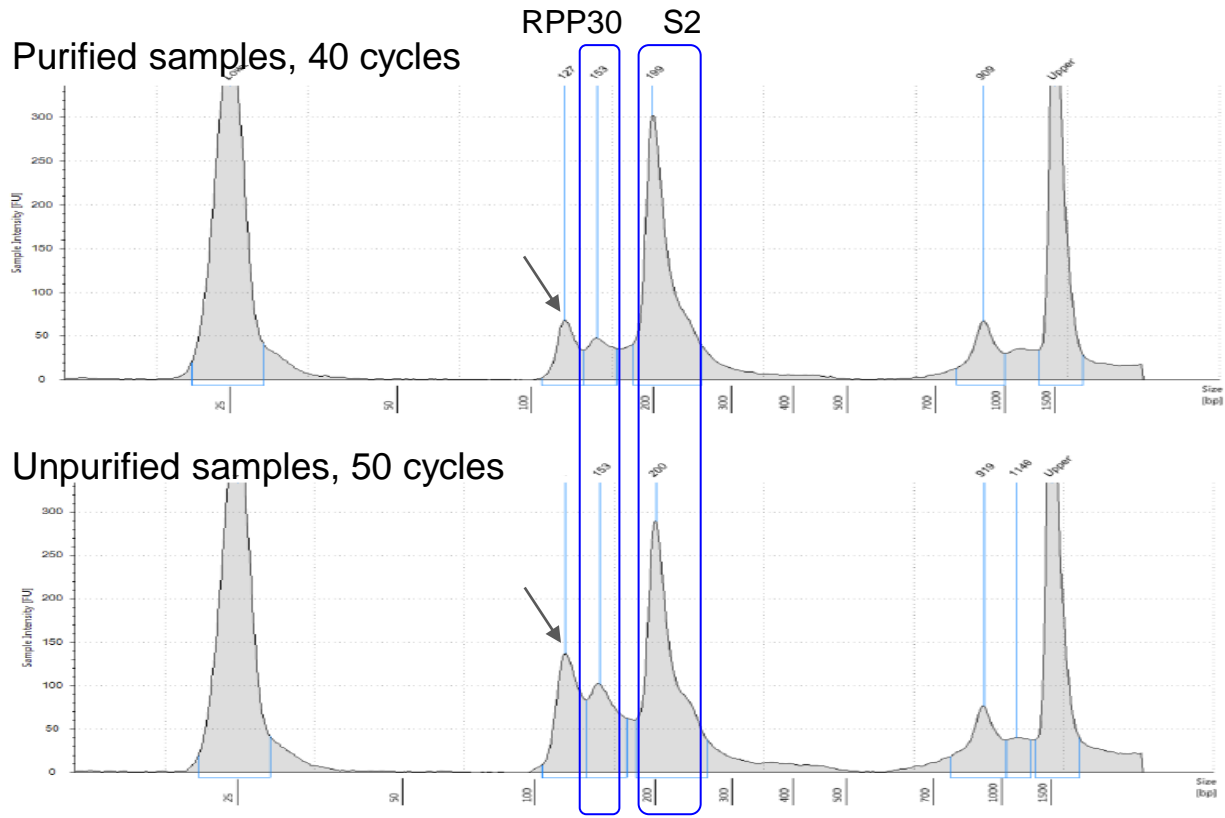
Figure S10. Tapestation Increasing the number of PCR cycles and working with unpurified or inhibitory samples types (eg. Saliva) was seen to increase the size of a nonspecific peak in our library preparation. Representative result from Agilent TapeStation for our purified amplicon libraries. We observe a nonspecific peak slightly above 100bp (arrow) in both library traces, but this peak increases in size with unpurified samples and an increased number of PCR cycles. While we have not confirmed the identity of this peak, we believe this peak may be the result of adapter dimers or unsequenceable PCR artifacts. Importantly, we observe that an increase in the size of this nonspecific peak leads to inaccurate library quantification. Therefore, in order to optimize cluster density on Illumina sequencers, we suggest quantifying the loading concentration of the final library based on the proportion of the desired peaks (RPP30 and S2).
