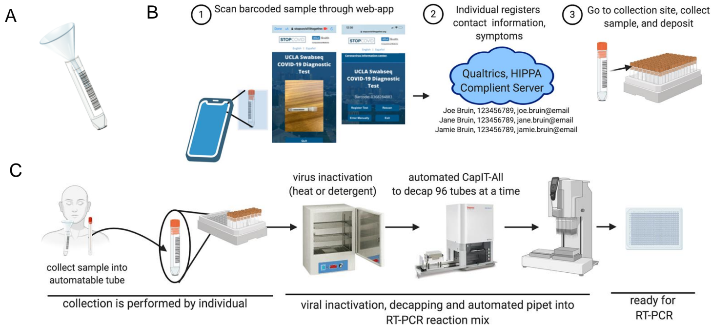
Figure S7. Developing a lightweight sample accessions, collection and processing to allow for scalable testing into the thousands of samples per day. A) To address the challenge of sample collection, we have developed lightweight collection methods that collect sample directly into an automatable tube. Here a funnel is used for an individual to deposit a small sample of saliva (0.25 mL into the funnel and tube). This setup can accommodate multiple sample types. B) To facilitate the sample accessions and collection, we developed a web-based app for individuals to register their sample tube using a barcode reader and send their identifying information into a secure instance of Qualtrics. Individuals then collect their sample and then place the tube in the rack. This low-touch pre-analytic process allows us to process thousands of samples a day without heavy administrative burden. C) The overall workflow streamlines processing in the lab. First, individuals collect samples into an automatable tube and place them into a 96-tube rack. Samples arrive in the lab in a 96-rack format allowing us to efficiently inactivate and process the samples, drastically increasing the flow of samples through our platform.
