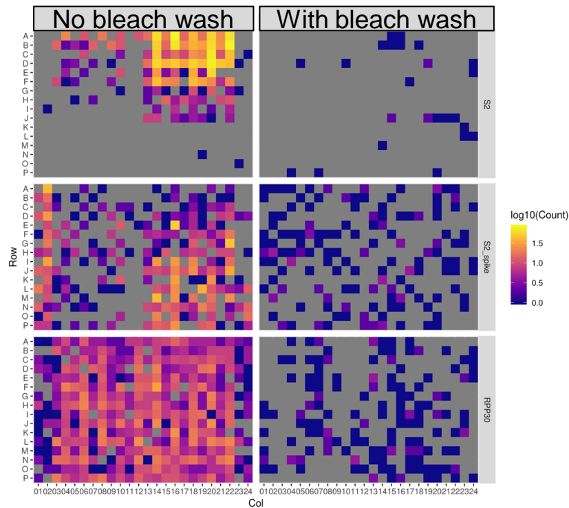
Figure S12. Carryover contamination from template line in a MiSeq contributes to cross contamination. In this experiment we did RT-PCR on four 384-well plates but only pooled three plates. On the left are observed counts of each of the amplicons for each sample for the 384-well plate not included in our run (but for which the indices were used in the previous run). Amplicon reads for indices used in the previous run are present at a low level (0-150 reads). We then performed a bleach wash in addition to regular wash prior to the subsequent run. In this subsequent run, we pooled three different plates and left out the fourth 384 well plate. On the right are observed counts of each of the amplicons for sample indices corresponding to the left-out plate (again, for which the indices were used in the previous run). We observe a remarkable decrease in the amount of carryover contamination, where carryover reads are <10 per sample.
