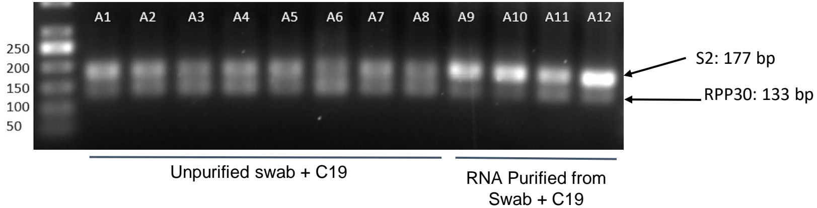
Figure S9. PCR inhibition has significant effect on amplification products. A) 2% Agarose gel was run for a subset of wells from our Rt-PCR reactions. We observe RT-PCR inhibition from swabs in unpurified lysate (A1-A8) as compared to purified RNA (A9-A12). We observe two bands in this subset of wells representing 2 amplicons for the S2 or S2 spike (177bp) and RPP30 (133 bp) primer pairs.
