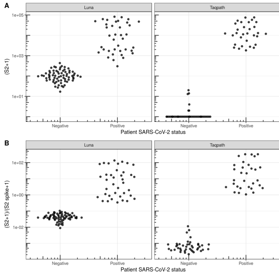
Figure S11. TaqPath decreases the number of S2 reads in SARS-CoV2-negative samples relative to NEB Luna. We compared Luna One Step RT-PCR Mix (New England Biosciences) to TaqPath™ 1-Step RT-qPCR Master Mix (Thermofisher Scientific). It is likely that the presence of UNG in the TaqPath Mastermix significantly reduced the number of S2 reads in the SARS-CoV-2-negative samples allowing us to more accurately distinguish SARS-CoV-2-positive and SARS-CoV-2-negative samples.
