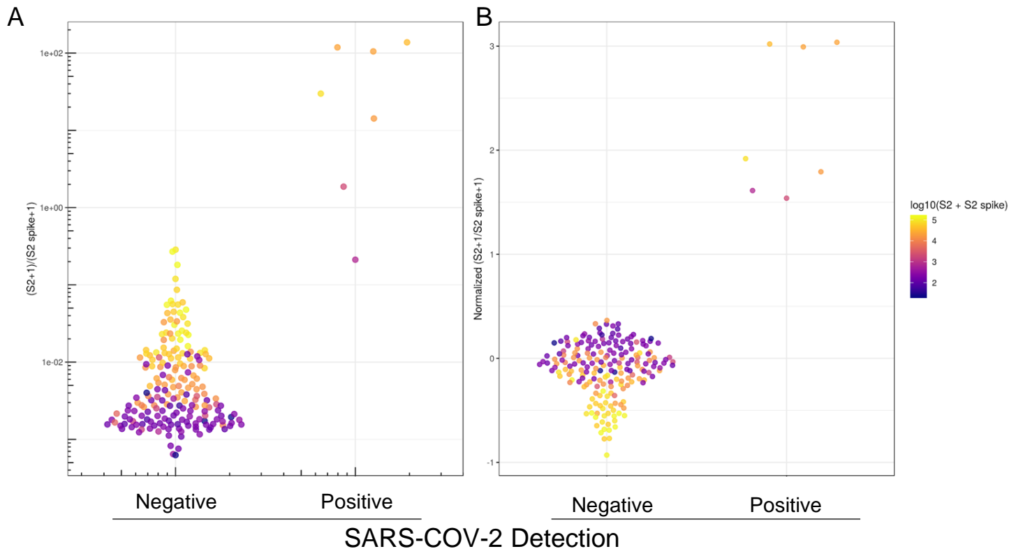
Figure S15. Computational correction for index mis-assignment using a mixed-model. To expand the number of samples we are capable of testing, we can use a combinatorial indexing strategy. In this experiment we used a single index on i5 to uniquely identify a plate and 96 i7 indices to identify wells. (A) The ratio of S2 to S2 spike (y-axis) is plotted for clinical samples based on whether Covid was detected by RT-qPCR (x-axis). SARS-CoV-2 positive samples were filtered to have Ct < 32 . The effects of index mis-assignment across plates can be observed as i7 indices that have high a sum of S2 and S2 spike across all samples that share the same i7 barcode across plates (colors). (B) Best linear unbiased predictor residuals are plotted (y-axis) for data in A, after computational correction of the \log_{10}(S2+1/S2\_spike+1) ratio by treating the identity of the i7 barcode as a random effect.
