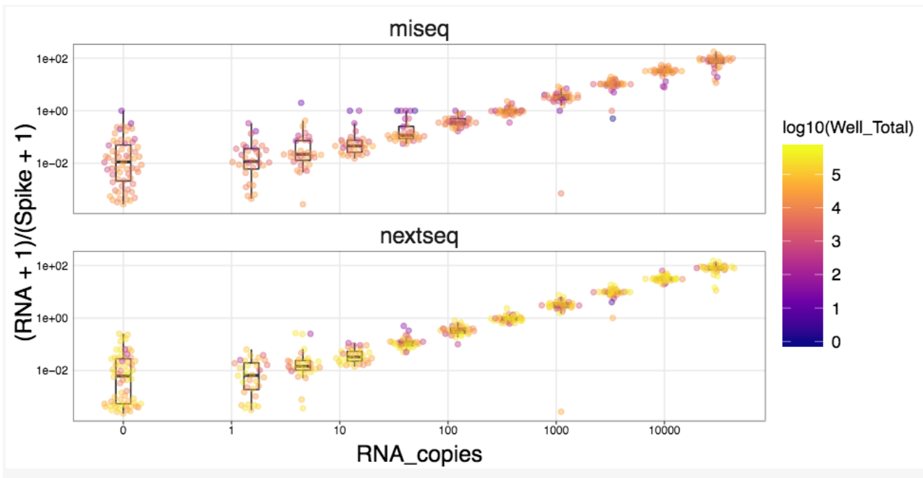
Figure S4. Sequencing is performed on MiSeq or NextSeq Machine with similar sensitivity. Multiplexed libraries run on both MiSeq and NextSeq showed linearity across a wide range of SARS-CoV2 virus copies in a purified RNA background.
