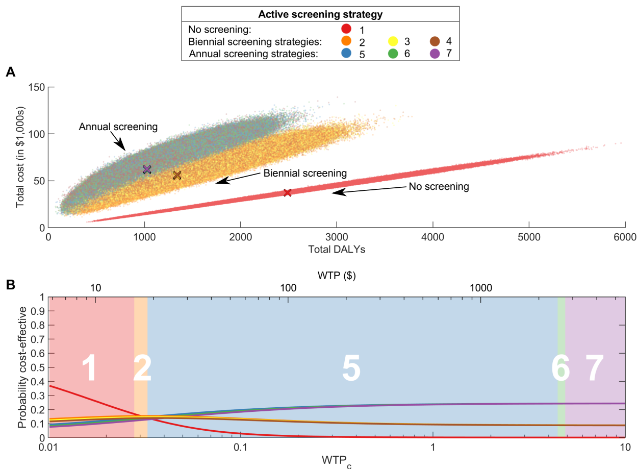
Figure 5: The cost-effectiveness of active screening strategies. (A) Cost-effectiveness plane showing the total cost of a strategy and the associated total number of DALYs. Mean values for each strategy are shown by the coloured crosses. (B) Cost-effectiveness acceptability curves (CEACs) for each strategy are shown by lines, with the cost-effectiveness acceptability frontier (CEAF) shown by the numbered background colour, which demonstrated the values for the ICER. WTP is shown in 2018 USD on the top and as the WTP_c coefficient on the bottom, where the coefficient is the multiplier of the GDP per capita of the DRC. See Table 2 for the full descriptions of the strategies.
