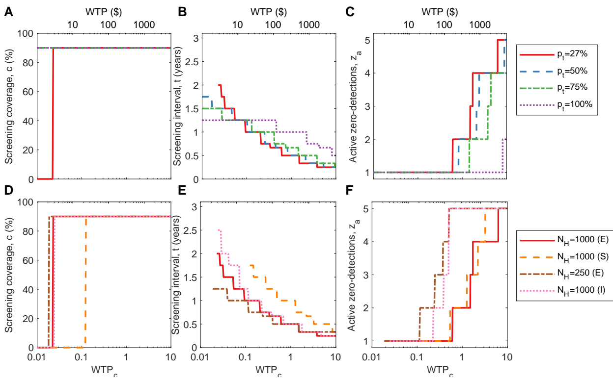
Figure 3: Theoretical optimum strategy for the mean simulation of infection dynamics given a range of WTP values (horizontal axis). (A)–(C) examine the impact of different treatment coverage ( p_t ) on (A) the optimal screening coverage, (B) the optimal screening interval and (C) the optimal number of zero-detections required to stop screening, to achieve the highest NMB for given WTP. These results assume a village population of 1,000 where the disease is endemic. (D)–(F) examine the impact of different assumptions about population size and endemicity on (D) the optimal screening coverage, (E) the optimal screening interval and (F) the optimal number of active zero-detections required to stop screening. The demography and disease endemicity assumptions are as follows: a population of population 1,000 where the disease is endemic (‘1000 (E)’), a village of population 1,000 where only one person is initially infected (single infection, or ‘1000 (S)’), a village of population 250 where disease is endemic (‘250 (E)’), and a village of population 1,000 where disease is endemic and there exists a small probability of infectious importations (‘1000 (I)’). We fix z_r = 1 for all simulations.
