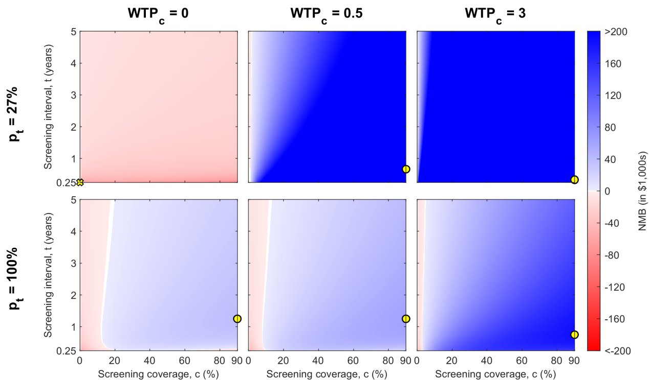
Figure 2: The mean NMB of different active screening strategies for given WTP per DALY averted (given as multiplication factor WTP_c of GDP per capita from the DRC) and the proportion of passive infections that are treated, p_t . The red areas show a negative NMB, while blue areas are positive NMB, with white at the boundary of no change. The maximum NMB for each WTP_c and p_t combination is marked by a yellow circle on each heatmap, with a cross if the maximum is for no active screening (only observed here for WTP_c = 0 and p_t = 27\% ). A population size of N_H = 1,000 is used and we fix z_a = 3 , the number of consecutive active screening rounds with zero-detections necessary to cease operations.
