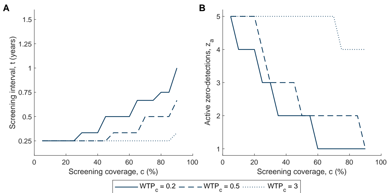
Figure 4: Optimal strategy given a maximum screening coverage informed by historic averages in the DRC. Results are shown for a WTP_c = 0.2, 0.5, 3 . z_r = 1 , p_t = 27\% , N_H = 1,000 are fixed and the optimum t and z_a is found simultaneously. (A) Optimal screening interval t . (B) Optimal number of zero-detections to stop screening z_a .
