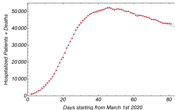
Figure 3b. The best fit curve represents the spreading in time of a wave packet in a dispersive medium according with the function (10) in the text.
