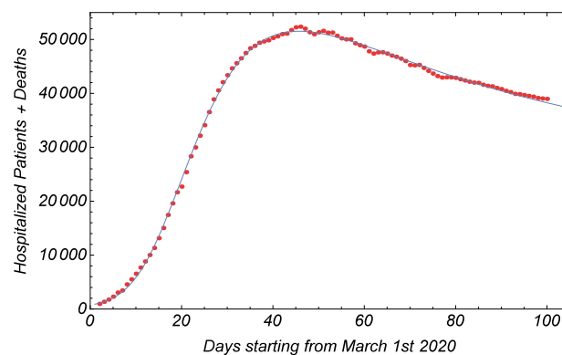
Figure 2b. Total number of Hospitalized Patients (Hospitalized Patients with symptoms and Patients in Intensive Care Units) and Deaths. Final fit: the best fit curve (Eq. (1) in the text) is obtained using 99 experimental points.
