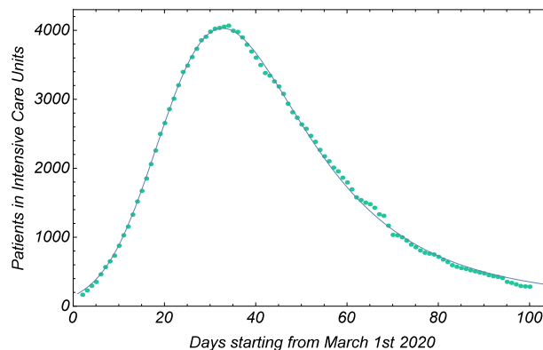
Figure 1b. Total number of patients in Intensive Care Units during the examined interval of time. Final fit: the best fit curve (Eq. (1) in the text) is obtained using 93 experimental points
