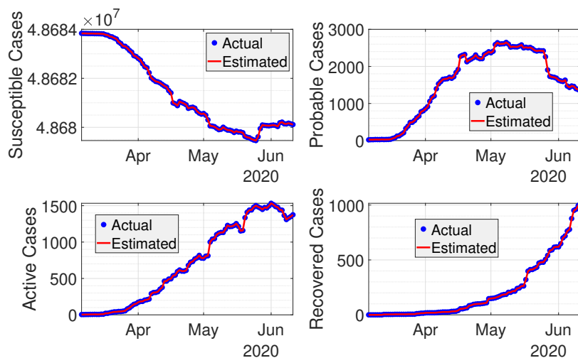
Figure 3: Real-time fitting using extended Kalman filter.
