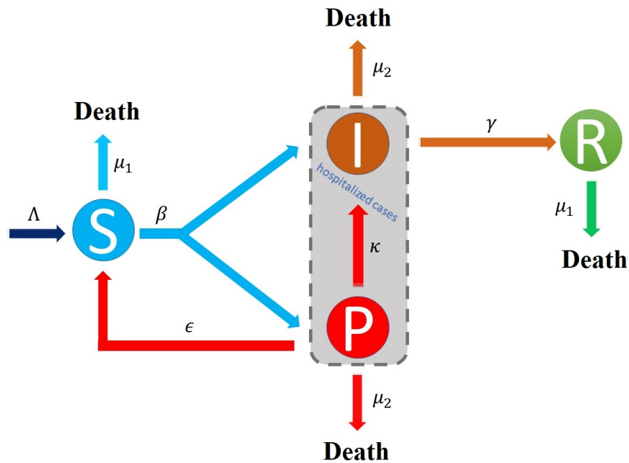
Figure 2: SPIR model is proposed to model probable cases of COVID-19 transmission process.
