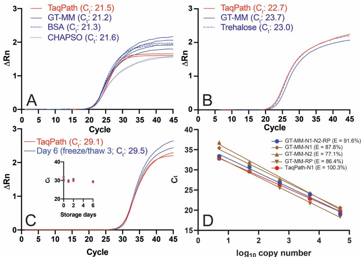
Figure 4. Performance of GT RT-qPCR master mix. RT-qPCRs were performed with the Georgia Tech thermal cycling conditions ( Table 2 ) and GT-Master Mix components ( Table 4 ) with ATCC synthetic viral RNA (ATCC® VR-3276SD™) and C_t values determined using a threshold of 0.1 unless otherwise noted. (A) Effect of CHAPSO (0.1%) and BSA (0.5 mg/mL) on GT master mix performance with IDT N1 primers and 50,000 copies of synthetic viral RNA. The no template control did not amplify. (B) Performance of GT multiplex primers and probes with 50,000 copies viral RNA with GT-Master Mix, compared to TaqPath, and effect of trehalose (9.5%). (C) Performance of GT-Master Mix (MM) with IDT N1 primers and 500 copies of synthetic viral RNA, compared to TaqPath, after three freeze/thaw cycles (six days of storage) at 2x concentration. Inset: C_t for GT-Master Mix and TaqPath over six days of storage. (D) qPCR efficiency ( E = 10^{-(1/\text{slope})} - 1 ) using auto threshold. GT-Master Mix and GT multiplex primers (N1 and N2 FAM readout, blue): 91.6%; GT-Master Mix and GT singleplex primers (brown): 87.8% for GT-N1 primer/probe (diamond), 77.1% GT-N2 primer/probe (triangle), 86.4% GT-RP primer/probe (inverted triangle); 100.3% TaqPath with GT-N1 primer/probe (red). Singleplex RT-qPCRs were performed with a mix of full-length viral RNA and HEK293T total RNA.
