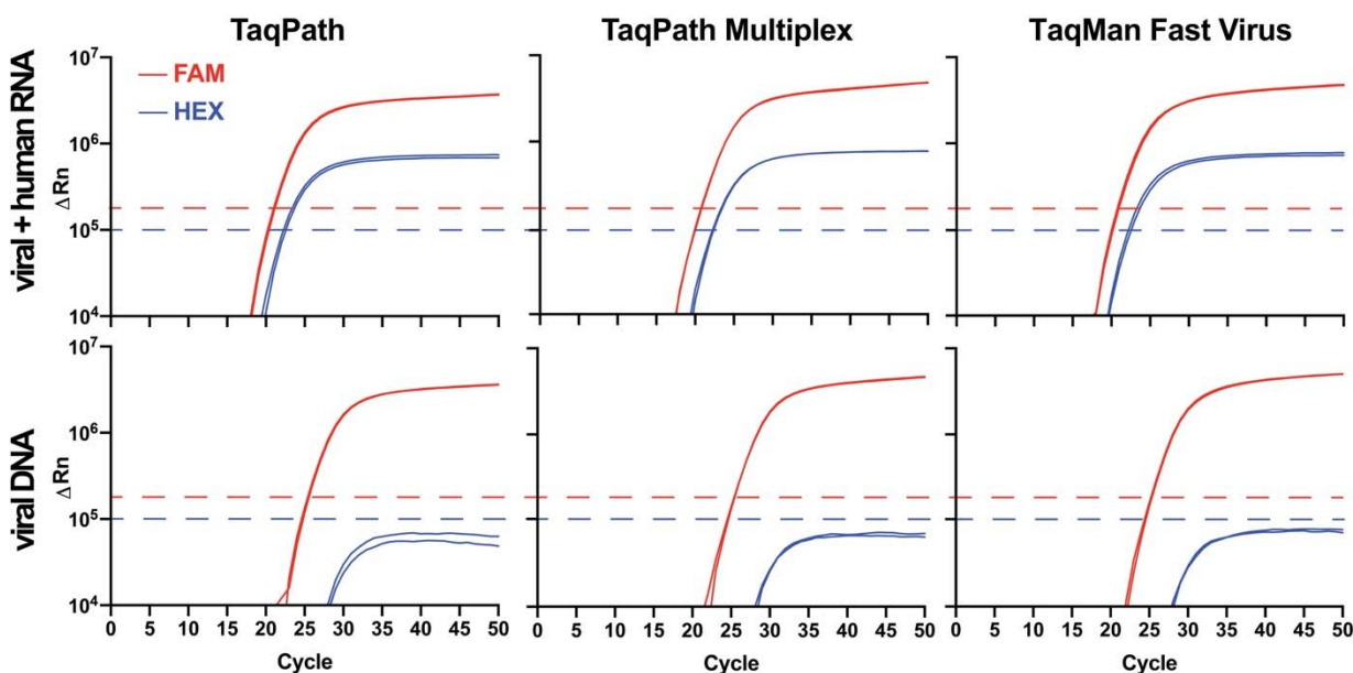
Figure 3. Performance of Georgia Tech multiplex primers and probes in several commercially available master mixes. GT multiplex primer/probe performance in commercial TaqPath, TaqPath Multiplex, and TaqMan Fast Virus 1-Step master mixes. Commercial master mix identity had no detectable impact on performance of the GT-made multiplex primer/probe mix. Due to the proximity of FAM and HEX channels, bleed-through from the FAM into the HEX channel was observed (see bottom nCov plasmid panels), but was of lower intensity than signal generated by the HEX-RP-BHQ1 probe (see top panels) and did not interfere with analyses when the HEX fluorescence threshold (blue dashed line) was set above the bleed-through noise. Template in the top row consisted of synthetic SARS-CoV-2 RNA (ATCC) mixed with HEK293T RNA. Results are consistent with those expected for a positive patient sample. A negative sample would consist of a single amplification curve in the HEX channel (blue line). Template in the bottom row was 2019_nCoV_N_Positive Control (IDT) plasmid DNA. Results are plotted logarithmically.
