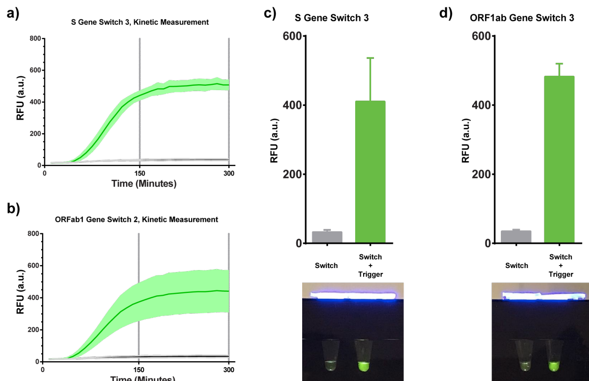
Figure 3: Characterization of S trigger/switch and ORF1ab trigger/switch couple in TXTL reaction. TXTL reactions were set-up in triplicates with addition of PCR amplified triggers and switch vectors. Reactions were monitored for 300 minutes with 10 minute intervals. Fluorescence measurements of a) S trigger/switch couple and b) ORF1ab trigger/switch couple. c) and d) Reaction results monitored using a DIY hand illuminator.
