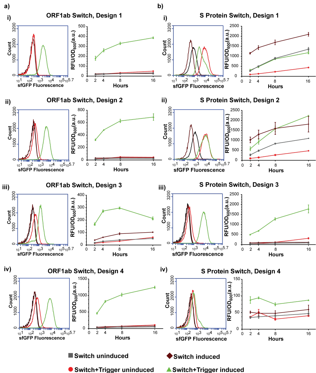
Figure 2: Characterization of best performing two trigger sequences found in S and ORF1ab region in vivo . For each trigger sequence, four different unique switch sequences were designed and cloned in p15A vector with T7 promoter and sfGFP coding sequence. Trigger sequences were cloned in ColE1 origin vectors with T7 promoter. Both vectors were transformed in BL21 (DE3) cells and induced. Flow cytometry results were taken after 90 minutes. Meanwhile, cells were monitored for 16 hours via total cell fluorescence measurements using a microplate reader. Cytometer results and total cell fluorescence measurements of designed switch for trigger sequence found in a) ORF1ab and b) S. For all microplate measurements, three replicates were used.
