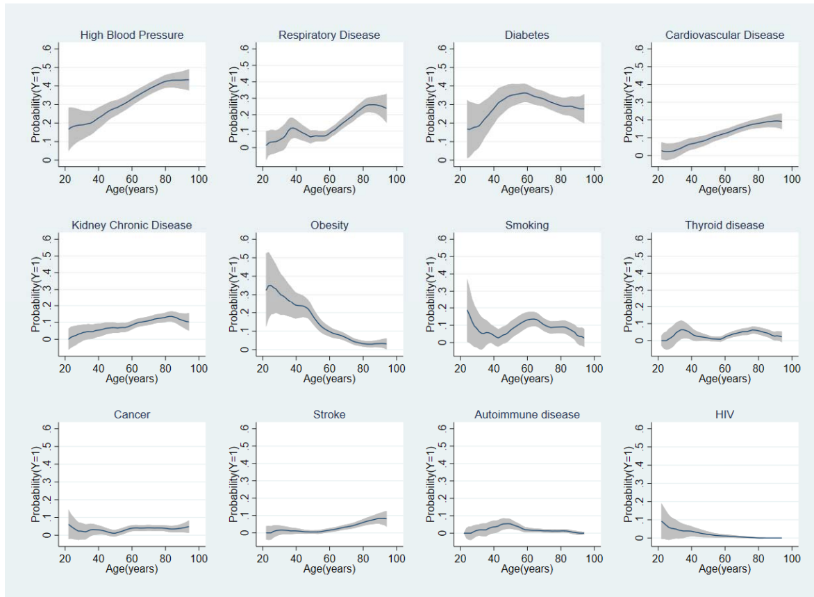
Figure 2. Locally weighted polynomial regressions between COVID-19, health condition and age, among fatal cases in Colombia. *
