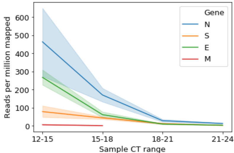
Supplemental Figure 1. sgRNA expression is correlated with CT range. Patient samples with lower CT values had significantly higher sub-genomic RNA (sgRNA) reads per million mapped (RPM) for genes E ( R^2=0.23 , p=1.4e-17 ), M ( R^2=0.17 , p=1.0e-03 ), and N ( R^2=0.02 , p=5.1e-03 ). These results show that our method is capable of sequencing SARS-CoV2 viral transcripts as well as genomes. Of note, proteins M and S were observed only in low-CT value samples.
