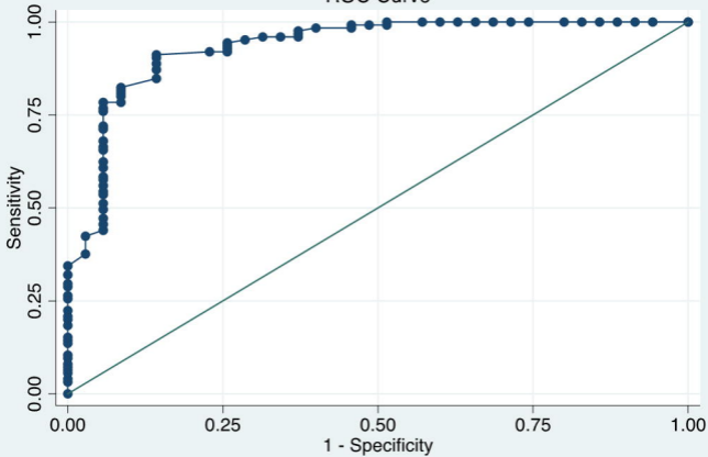
ROC Curve
