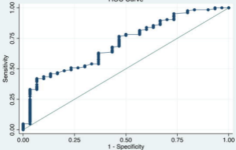
ROC Curve
